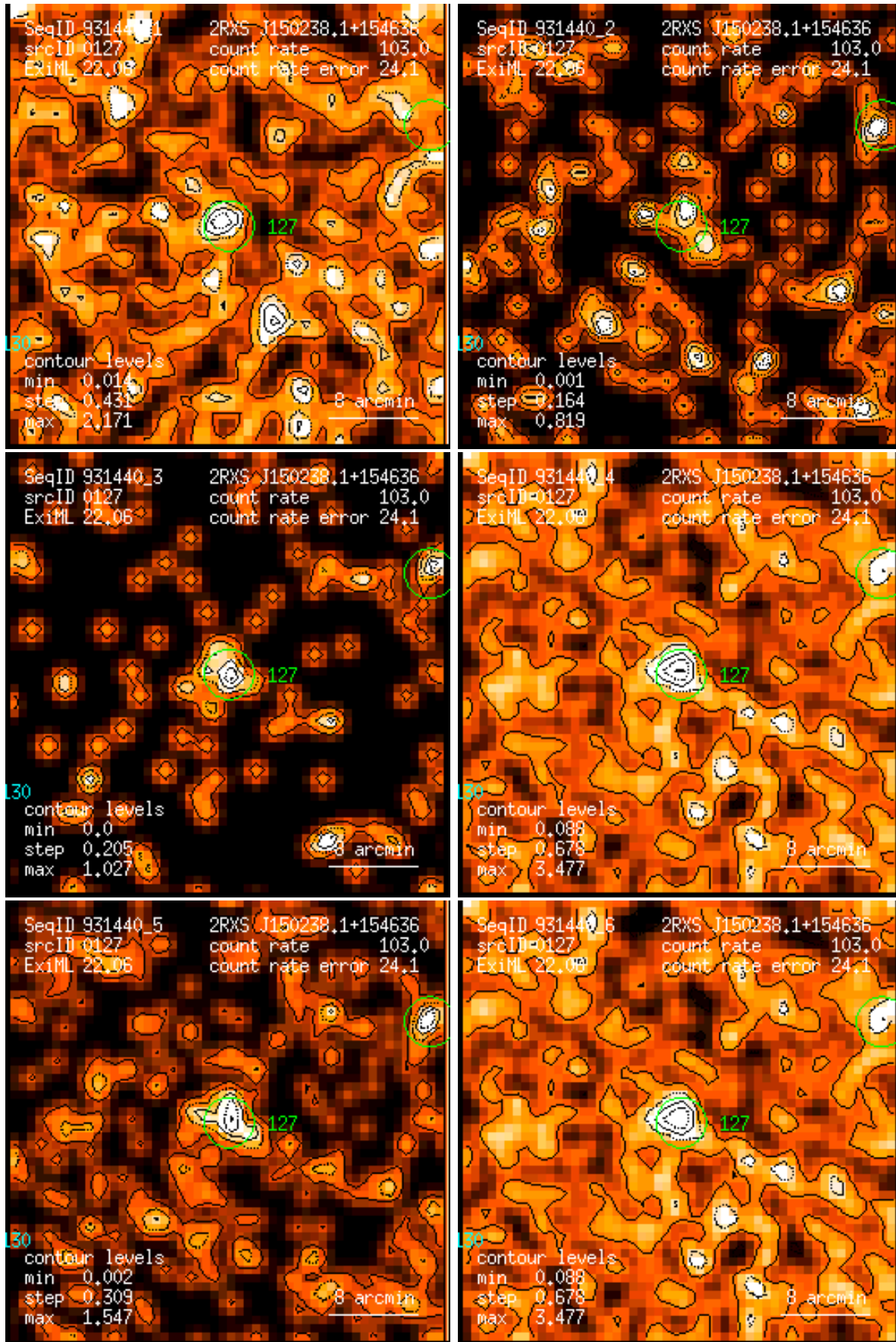
Figure 127: RASS 931440: detection 0127: band rate images, Gaussian filter: (1) PSPC channels 11 – 41, (2) 52 – 90, (3) 91 – 201, (4) 11 – 235, (5) 52 – 201, (6) 11 – 201. Broad band rates in counts/ks. Band rate contour levels in counts/ks/arcmin 2 .
