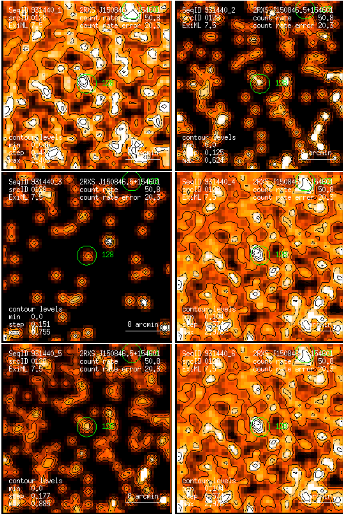
Figure 128: RASS 931440: detection 0128: band rate images, Gaussian filter: (1) PSPC channels 11 – 41, (2) 52 – 90, (3) 91 – 201, (4) 11 – 235, (5) 52 – 201, (6) 11 – 201. Broad band rates in counts/ks. Band rate contour levels in counts/ks/arcmin 2 .
