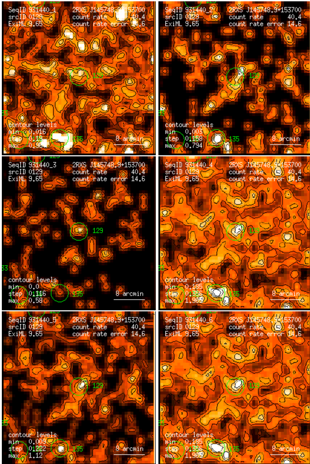
Figure 129: RASS 931440: detection 0129: band rate images, Gaussian filter: (1) PSPC channels 11 – 41, (2) 52 – 90, (3) 91 – 201, (4) 11 – 235, (5) 52 – 201, (6) 11 – 201. Broad band rates in counts/ks. Band rate contour levels in counts/ks/arcmin 2 .
