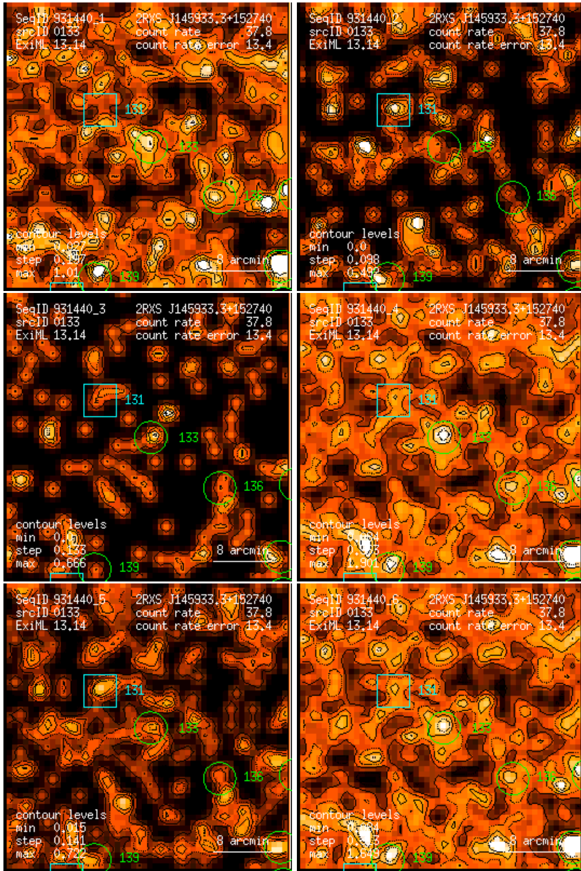
Figure 133: RASS 931440: detection 0133: band rate images, Gaussian filter: (1) PSPC channels 11 – 41, (2) 52 – 90, (3) 91 – 201, (4) 11 – 235, (5) 52 – 201, (6) 11 – 201. Broad band rates in counts/ks. Band rate contour levels in counts/ks/arcmin 2 .
