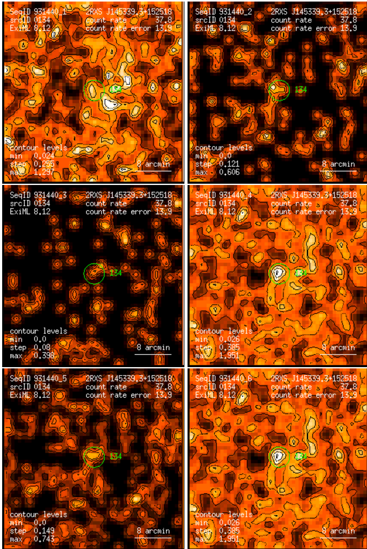
Figure 134: RASS 931440: detection 0134: band rate images, Gaussian filter: (1) PSPC channels 11 – 41, (2) 52 – 90, (3) 91 – 201, (4) 11 – 235, (5) 52 – 201, (6) 11 – 201. Broad band rates in counts/ks. Band rate contour levels in counts/ks/arcmin 2 .
