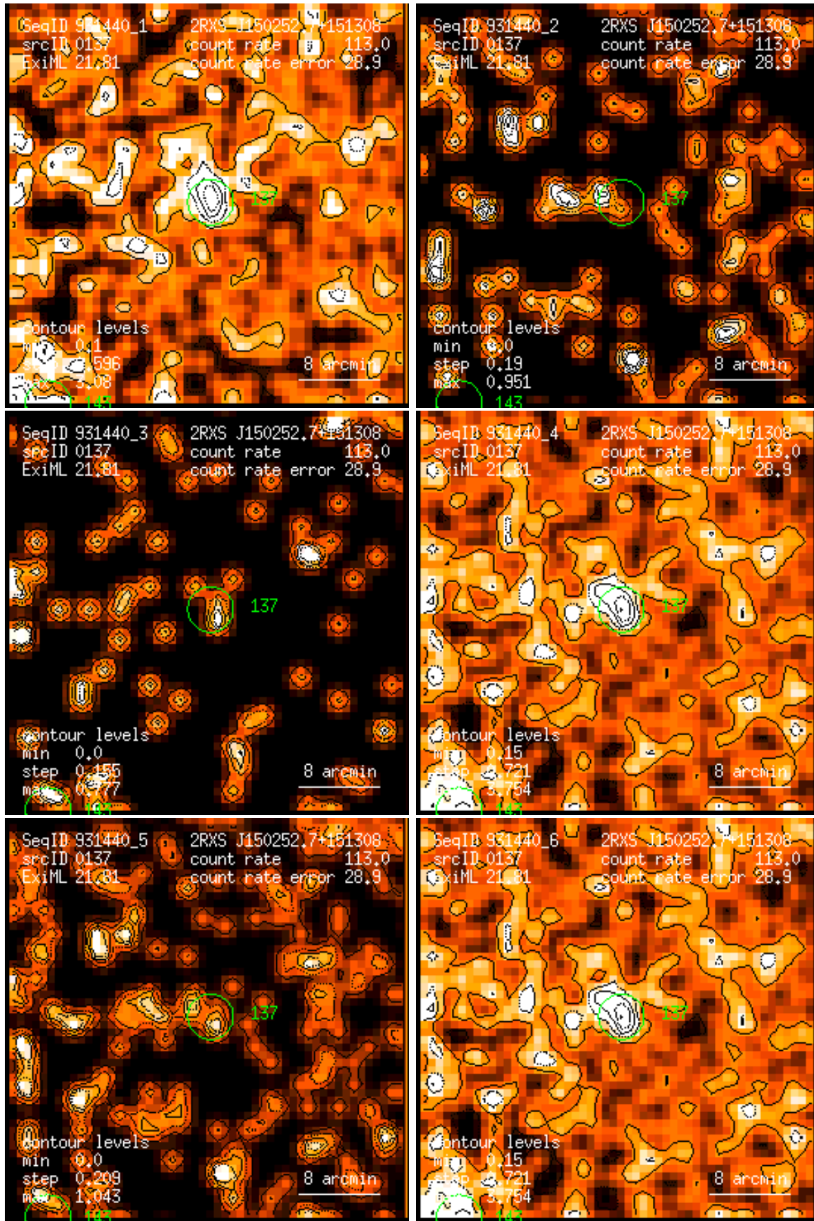
Figure 137: RASS 931440: detection 0137: band rate images, Gaussian filter: (1) PSPC channels 11 – 41, (2) 52 – 90, (3) 91 – 201, (4) 11 – 235, (5) 52 – 201, (6) 11 – 201. Broad band rates in counts/ks. Band rate contour levels in counts/ks/arcmin 2 .
