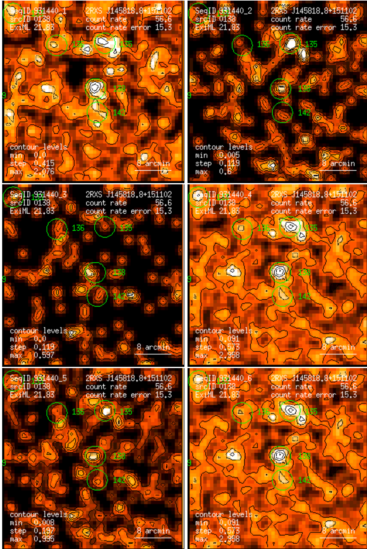
Figure 138: RASS 931440: detection 0138: band rate images, Gaussian filter: (1) PSPC channels 11 – 41, (2) 52 – 90, (3) 91 – 201, (4) 11 – 235, (5) 52 – 201, (6) 11 – 201. Broad band rates in counts/ks. Band rate contour levels in counts/ks/arcmin 2 .
