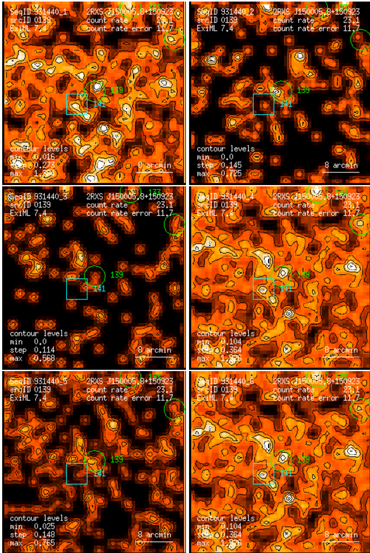
Figure 139: RASS 931440: detection 0139: band rate images, Gaussian filter: (1) PSPC channels 11 – 41, (2) 52 – 90, (3) 91 – 201, (4) 11 – 235, (5) 52 – 201, (6) 11 – 201. Broad band rates in counts/ks. Band rate contour levels in counts/ks/arcmin 2 .
