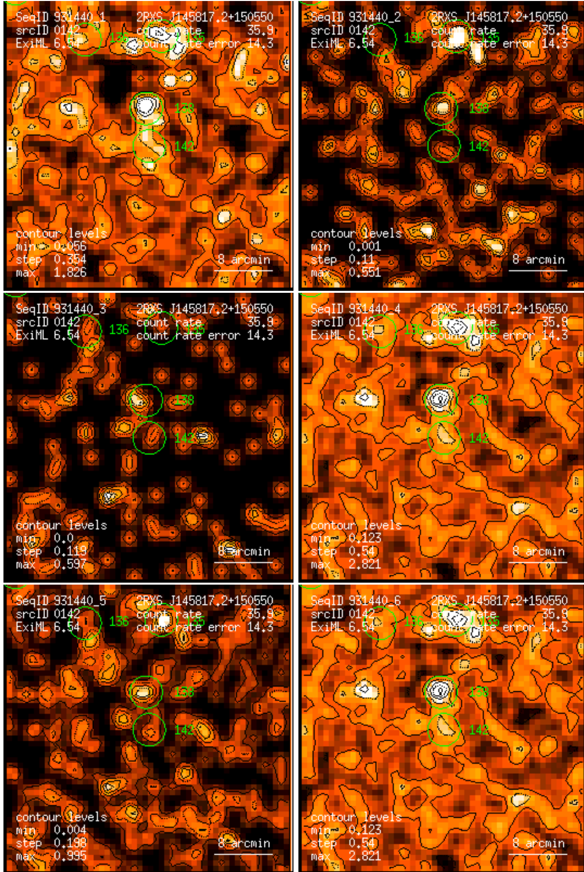
Figure 142: RASS 931440: detection 0142: band rate images, Gaussian filter: (1) PSPC channels 11 – 41, (2) 52 – 90, (3) 91 – 201, (4) 11 – 235, (5) 52 – 201, (6) 11 – 201. Broad band rates in counts/ks. Band rate contour levels in counts/ks/arcmin 2 .
