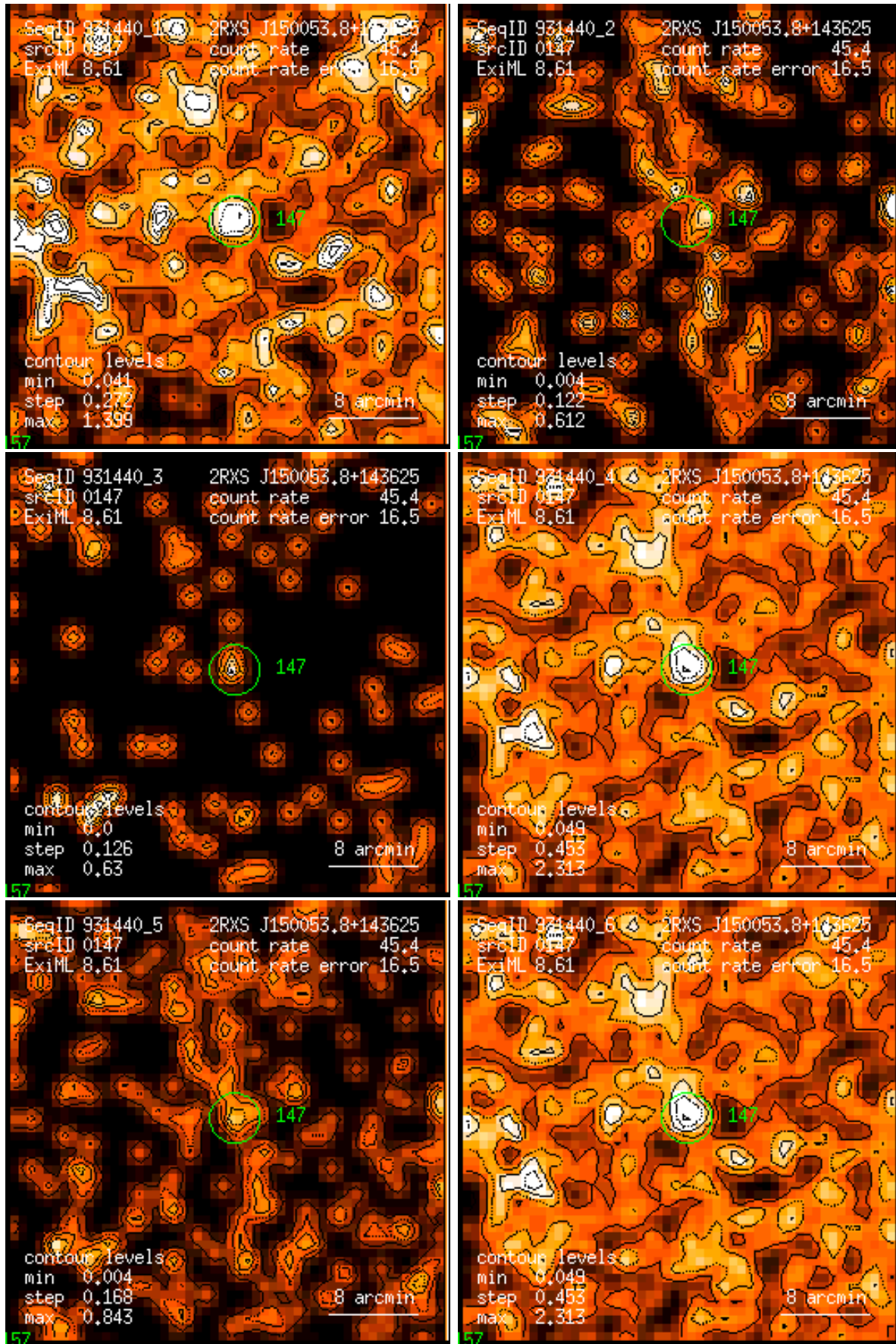
Figure 147: RASS 931440: detection 0147: band rate images, Gaussian filter: (1) PSPC channels 11 – 41, (2) 52 – 90, (3) 91 – 201, (4) 11 – 235, (5) 52 – 201, (6) 11 – 201. Broad band rates in counts/ks. Band rate contour levels in counts/ks/arcmin 2 .
