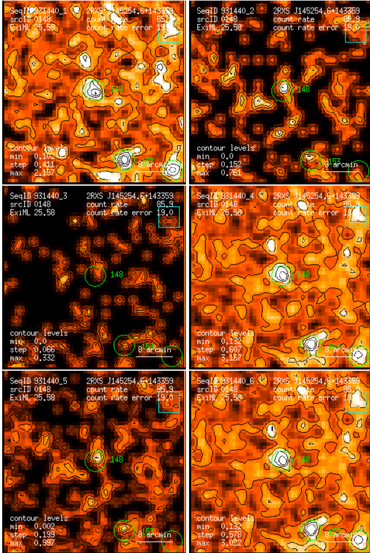
Figure 148: RASS 931440: detection 0148: band rate images, Gaussian filter: (1) PSPC channels 11 – 41, (2) 52 – 90, (3) 91 – 201, (4) 11 – 235, (5) 52 – 201, (6) 11 – 201. Broad band rates in counts/ks. Band rate contour levels in counts/ks/arcmin 2 .
