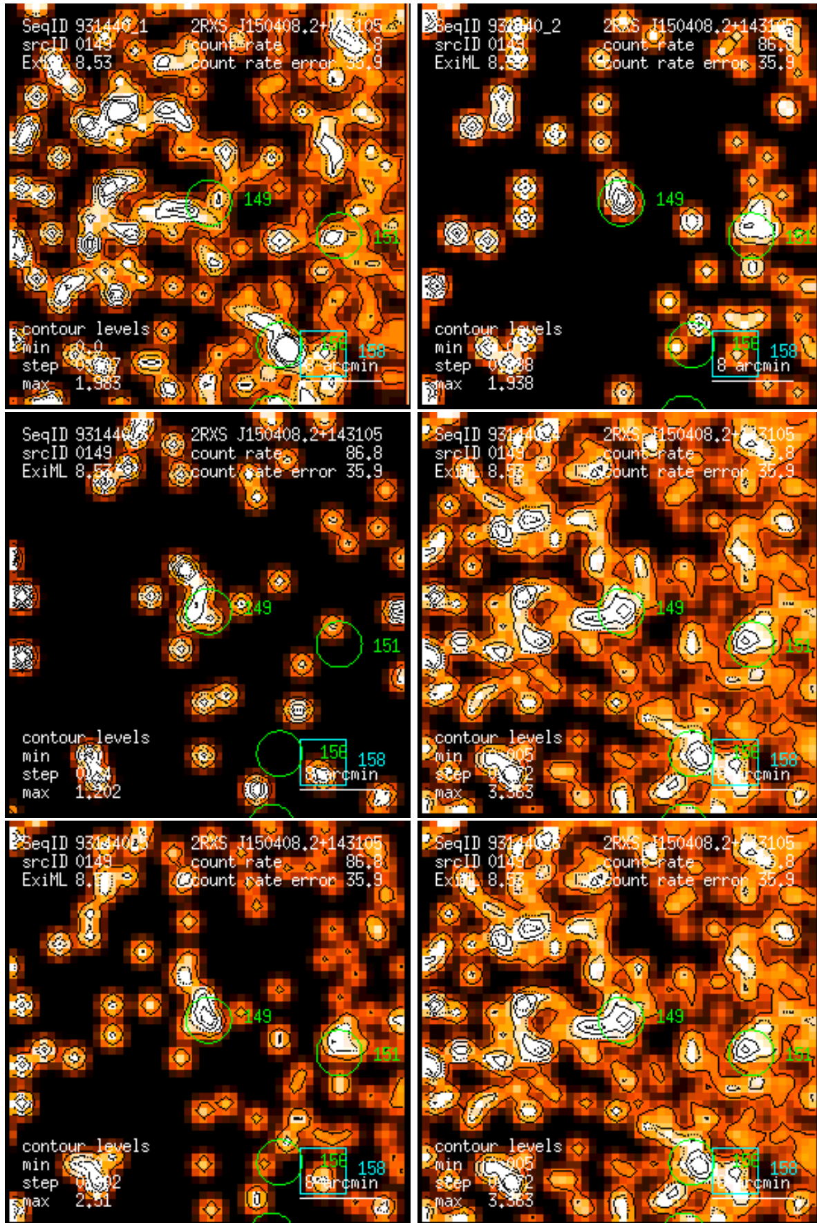
Figure 149: RASS 931440: detection 0149: band rate images, Gaussian filter: (1) PSPC channels 11 – 41, (2) 52 – 90, (3) 91 – 201, (4) 11 – 235, (5) 52 – 201, (6) 11 – 201. Broad band rates in counts/ks. Band rate contour levels in counts/ks/arcmin 2 .
