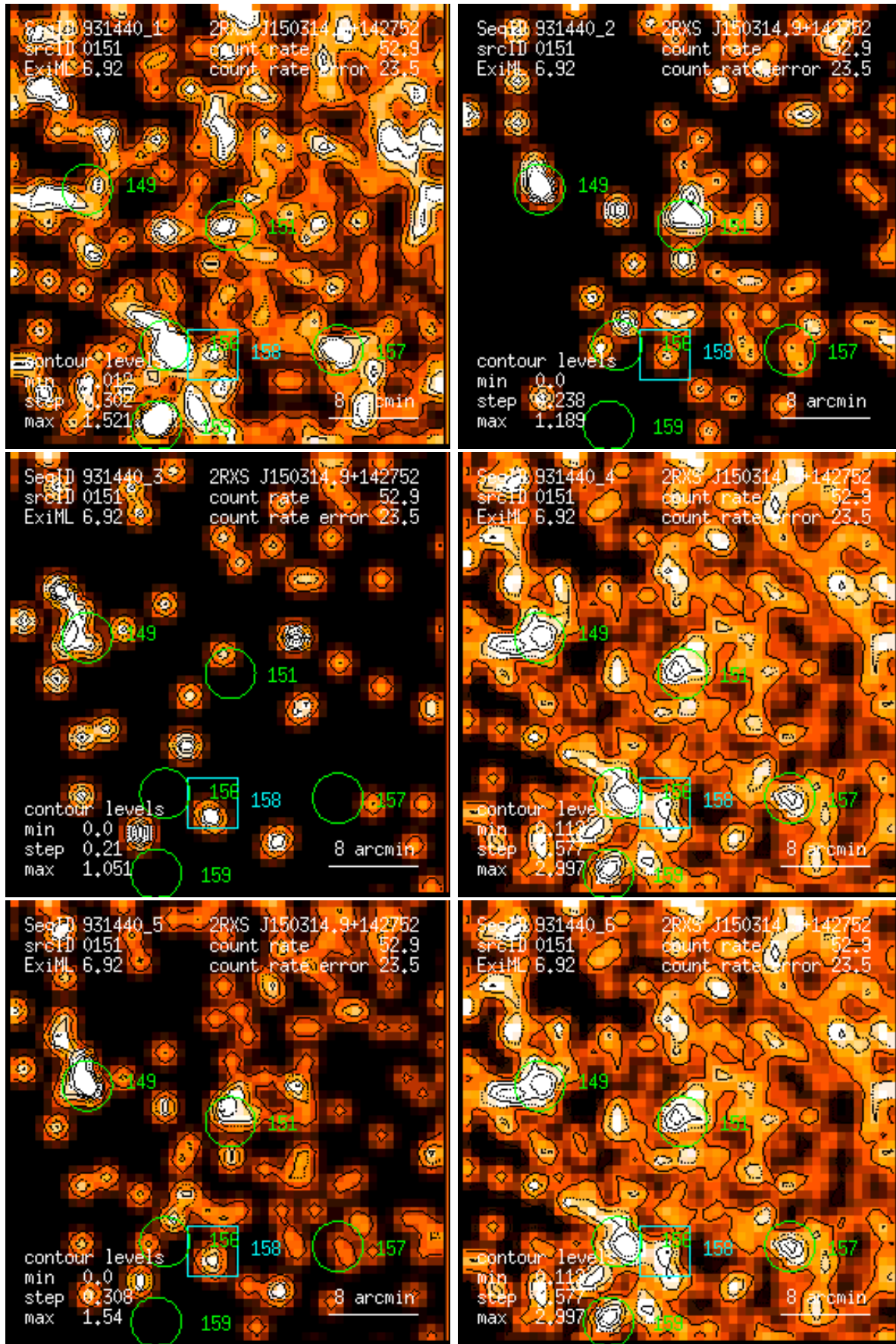
Figure 151: RASS 931440: detection 0151: band rate images, Gaussian filter: (1) PSPC channels 11 – 41, (2) 52 – 90, (3) 91 – 201, (4) 11 – 235, (5) 52 – 201, (6) 11 – 201. Broad band rates in counts/ks. Band rate contour levels in counts/ks/arcmin 2 .
