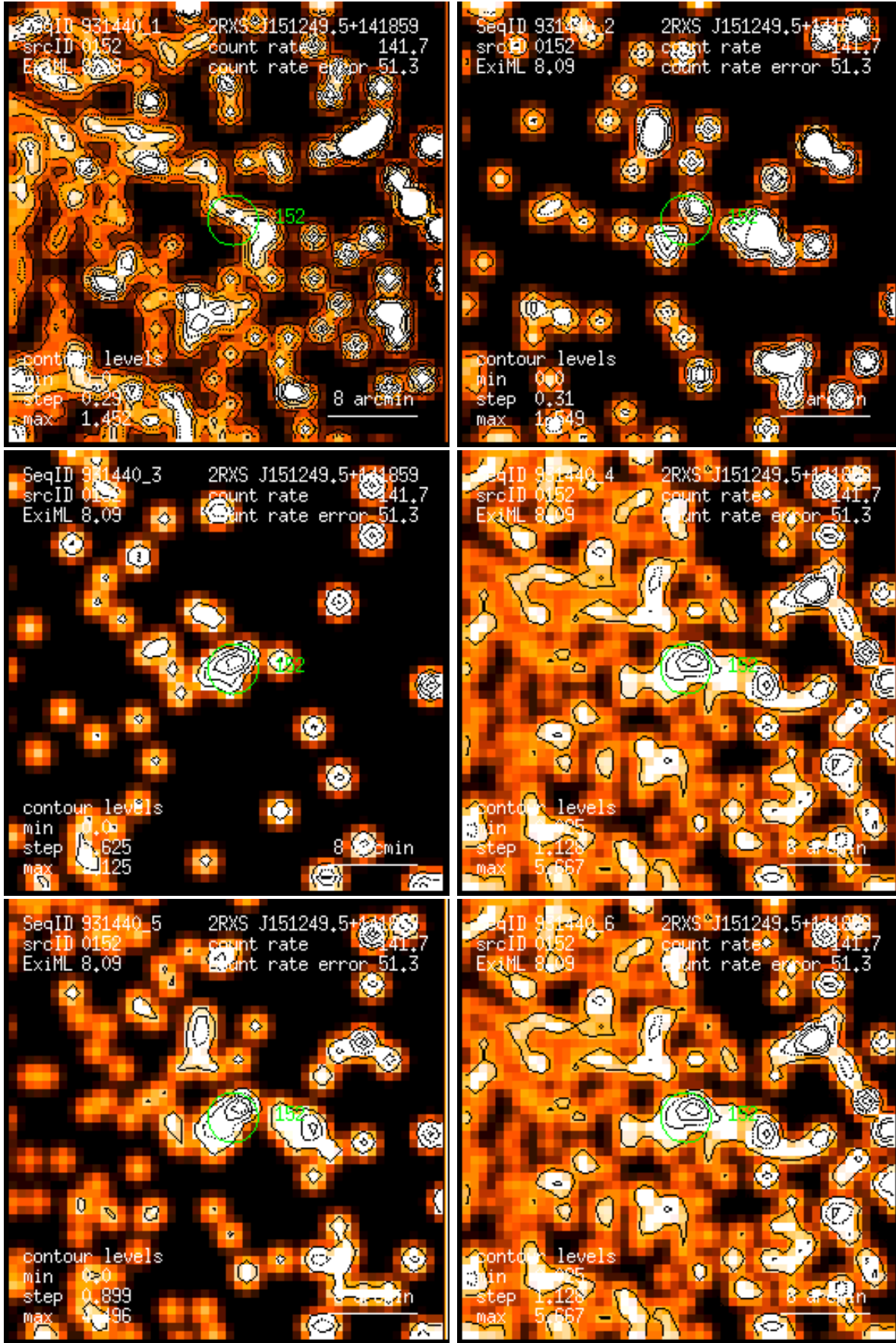
Figure 152: RASS 931440: detection 0152: band rate images, Gaussian filter: (1) PSPC channels 11 – 41, (2) 52 – 90, (3) 91 – 201, (4) 11 – 235, (5) 52 – 201, (6) 11 – 201. Broad band rates in counts/ks. Band rate contour levels in counts/ks/arcmin 2 .
