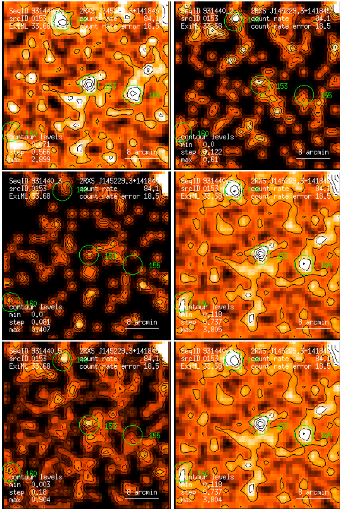
Figure 153: RASS 931440: detection 0153: band rate images, Gaussian filter: (1) PSPC channels 11 – 41, (2) 52 – 90, (3) 91 – 201, (4) 11 – 235, (5) 52 – 201, (6) 11 – 201. Broad band rates in counts/ks. Band rate contour levels in counts/ks/arcmin 2 .
