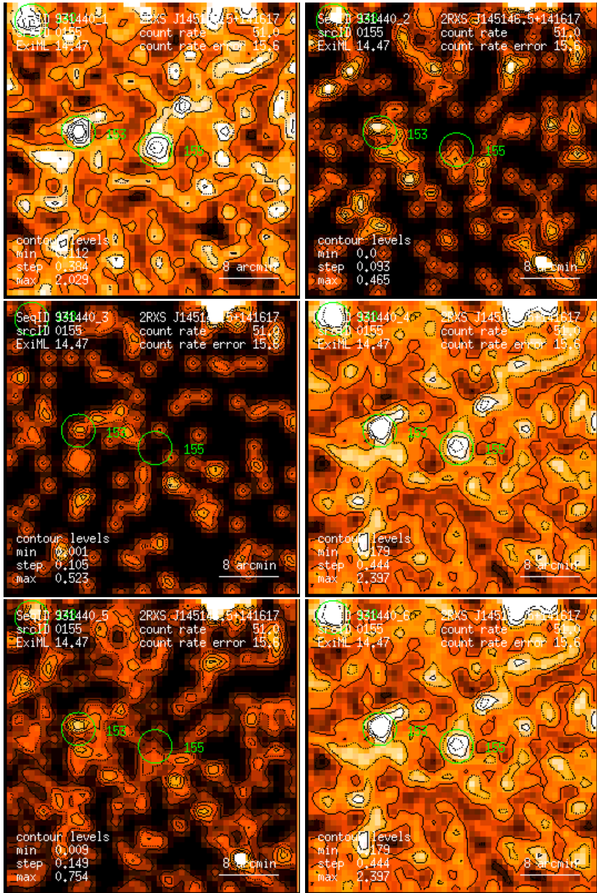
Figure 155: RASS 931440: detection 0155: band rate images, Gaussian filter: (1) PSPC channels 11 – 41, (2) 52 – 90, (3) 91 – 201, (4) 11 – 235, (5) 52 – 201, (6) 11 – 201. Broad band rates in counts/ks. Band rate contour levels in counts/ks/arcmin 2 .
