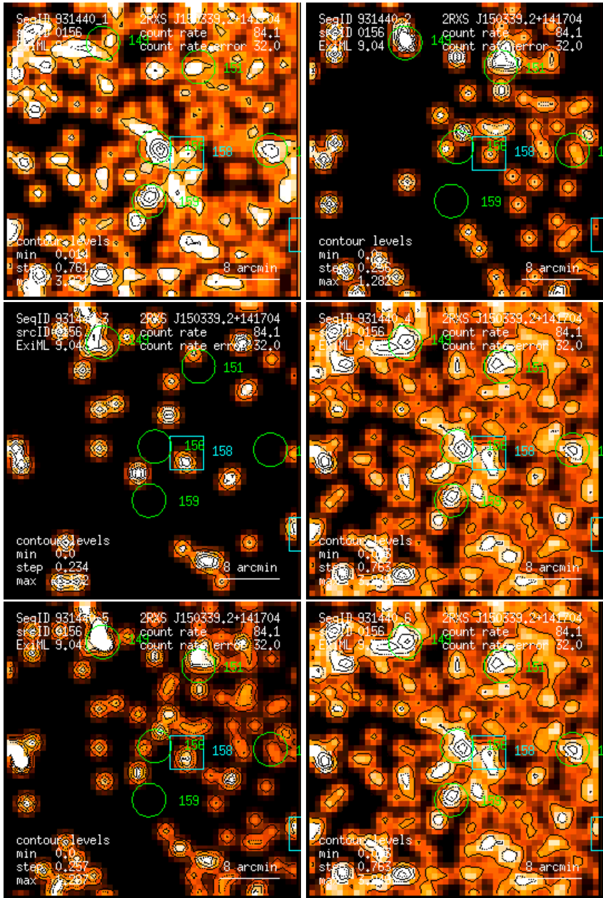
Figure 156: RASS 931440: detection 0156: band rate images, Gaussian filter: (1) PSPC channels 11 – 41, (2) 52 – 90, (3) 91 – 201, (4) 11 – 235, (5) 52 – 201, (6) 11 – 201. Broad band rates in counts/ks. Band rate contour levels in counts/ks/arcmin 2 .
