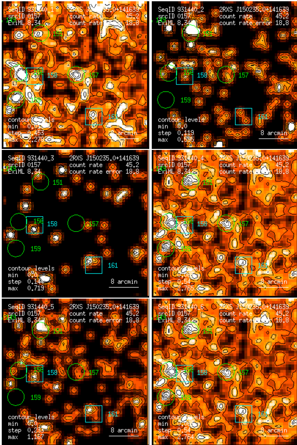
Figure 157: RASS 931440: detection 0157: band rate images, Gaussian filter: (1) PSPC channels 11 – 41, (2) 52 – 90, (3) 91 – 201, (4) 11 – 235, (5) 52 – 201, (6) 11 – 201. Broad band rates in counts/ks. Band rate contour levels in counts/ks/arcmin 2 .
