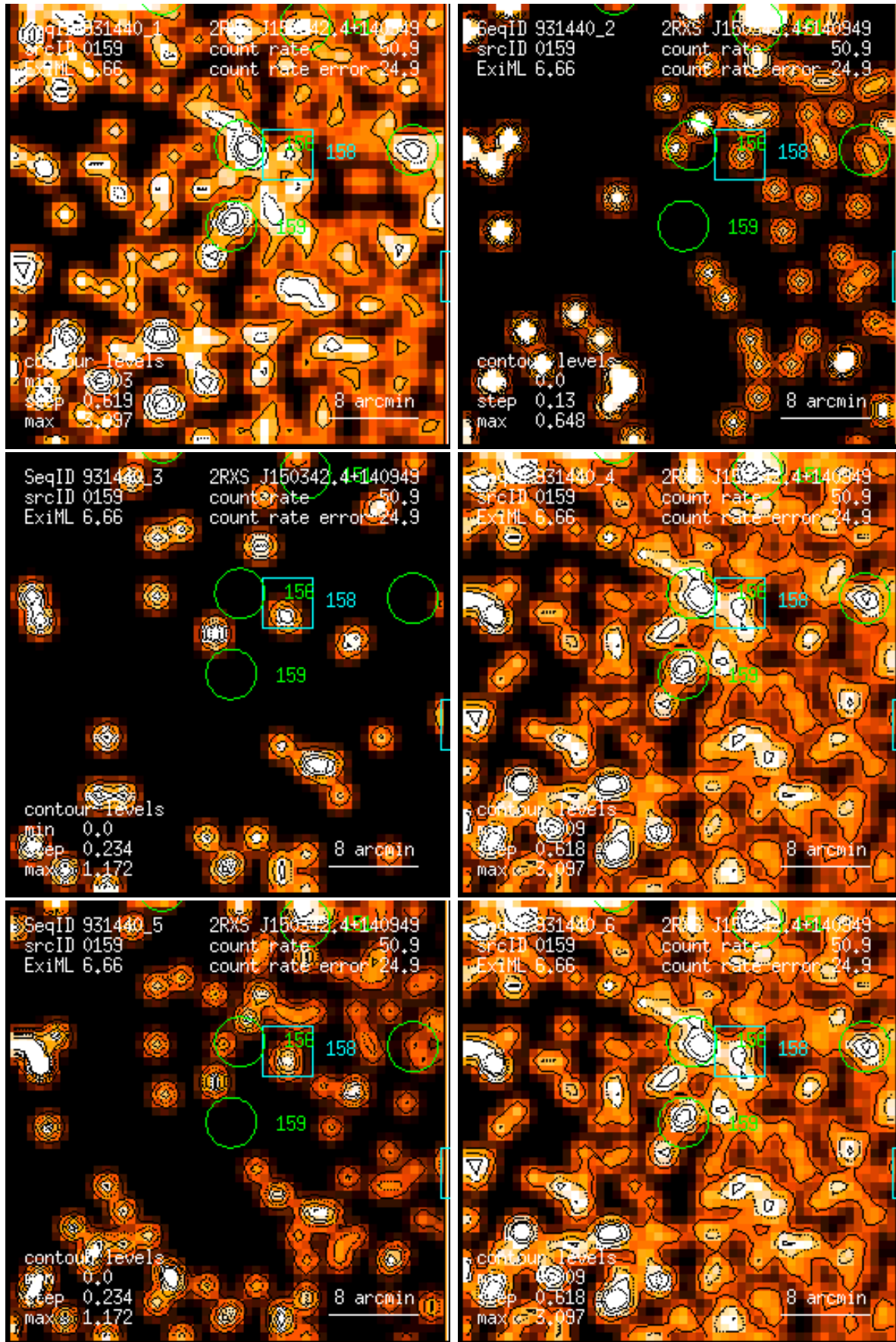
Figure 159: RASS 931440: detection 0159: band rate images, Gaussian filter: (1) PSPC channels 11 – 41, (2) 52 – 90, (3) 91 – 201, (4) 11 – 235, (5) 52 – 201, (6) 11 – 201. Broad band rates in counts/ks. Band rate contour levels in counts/ks/arcmin 2 .
