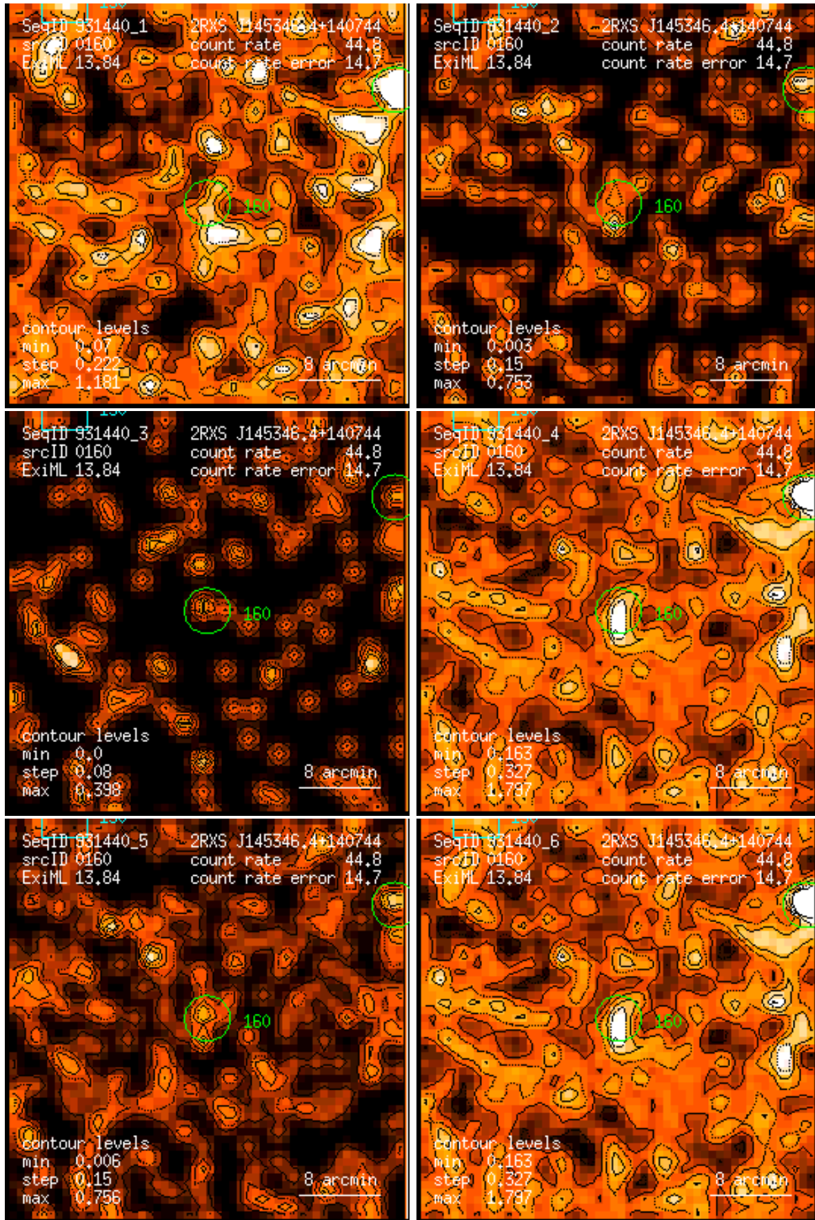
Figure 160: RASS 931440: detection 0160: band rate images, Gaussian filter: (1) PSPC channels 11 – 41, (2) 52 – 90, (3) 91 – 201, (4) 11 – 235, (5) 52 – 201, (6) 11 – 201. Broad band rates in counts/ks. Band rate contour levels in counts/ks/arcmin 2 .
