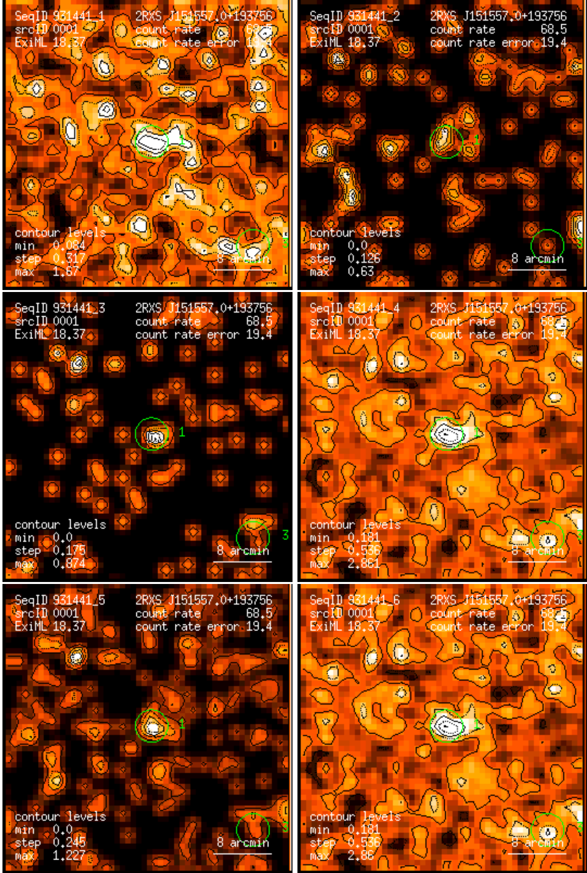
Figure 1: RASS 931441: detection 0001: band rate images, Gaussian filter: (1) PSPC channels 11 – 41, (2) 52 – 90, (3) 91 – 201, (4) 11 – 235, (5) 52 – 201, (6) 11 – 201. Broad band rates in counts/ks. Band rate contour levels in counts/ks/arcmin 2 .
