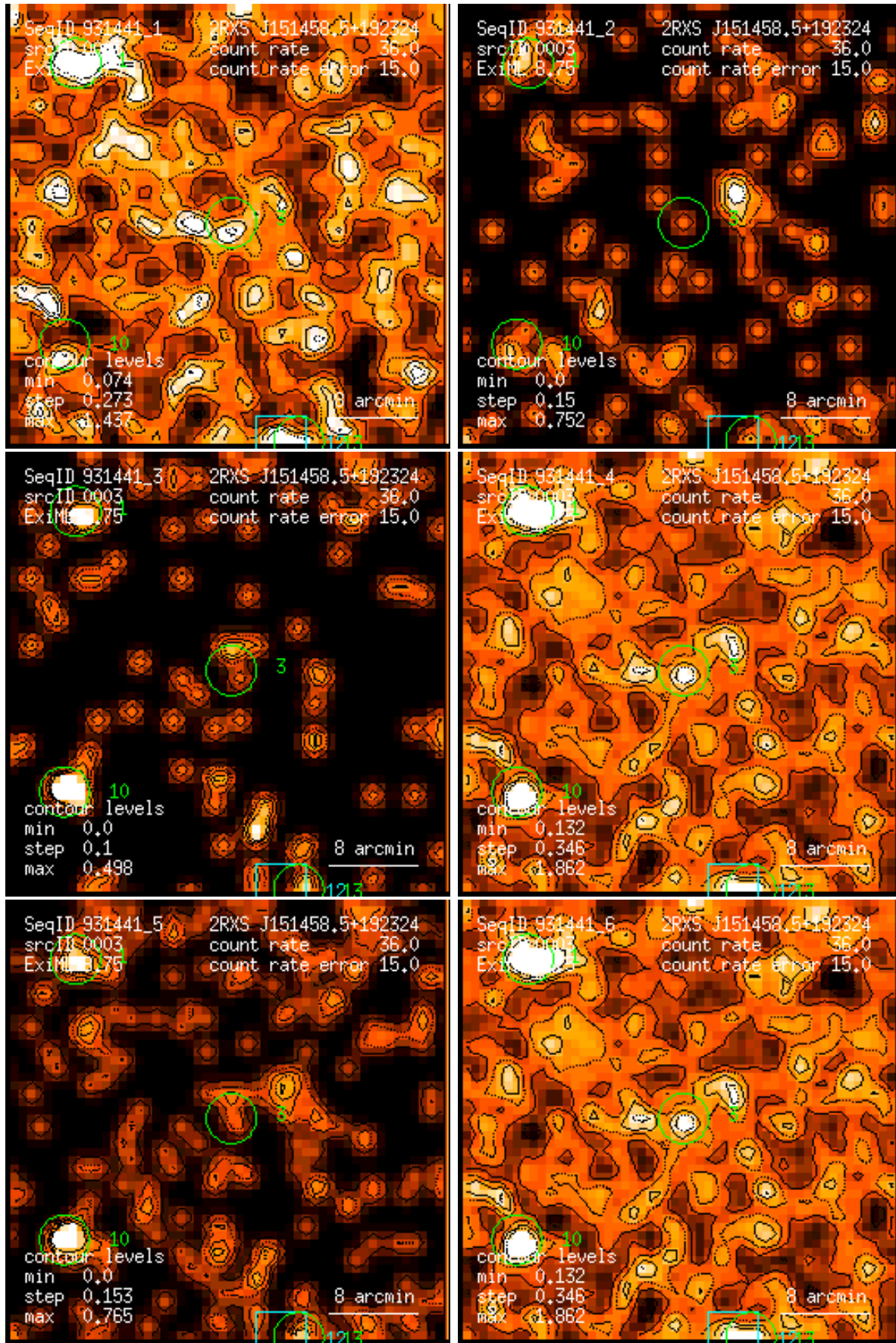
Figure 3: RASS 931441: detection 0003: band rate images, Gaussian filter: (1) PSPC channels 11 – 41, (2) 52 – 90, (3) 91 – 201, (4) 11 – 235, (5) 52 – 201, (6) 11 – 201. Broad band rates in counts/ks. Band rate contour levels in counts/ks/arcmin 2 .
