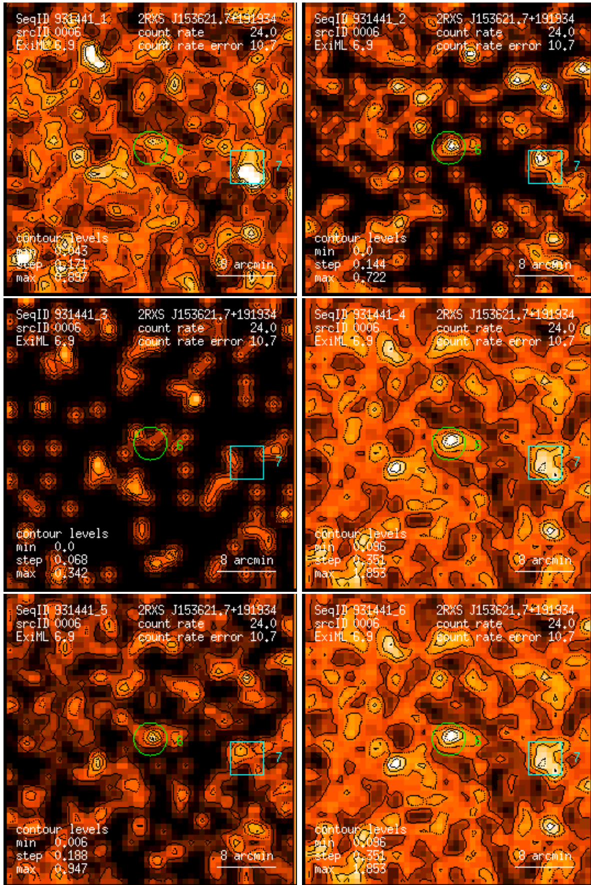
Figure 6: RASS 931441: detection 0006: band rate images, Gaussian filter: (1) PSPC channels 11 – 41, (2) 52 – 90, (3) 91 – 201, (4) 11 – 235, (5) 52 – 201, (6) 11 – 201. Broad band rates in counts/ks. Band rate contour levels in counts/ks/arcmin 2 .
