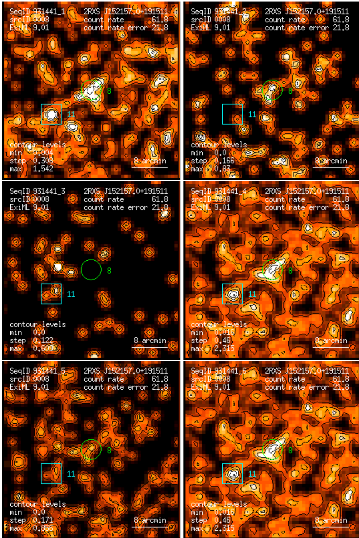
Figure 8: RASS 931441: detection 0008: band rate images, Gaussian filter: (1) PSPC channels 11 – 41, (2) 52 – 90, (3) 91 – 201, (4) 11 – 235, (5) 52 – 201, (6) 11 – 201. Broad band rates in counts/ks. Band rate contour levels in counts/ks/arcmin 2 .
