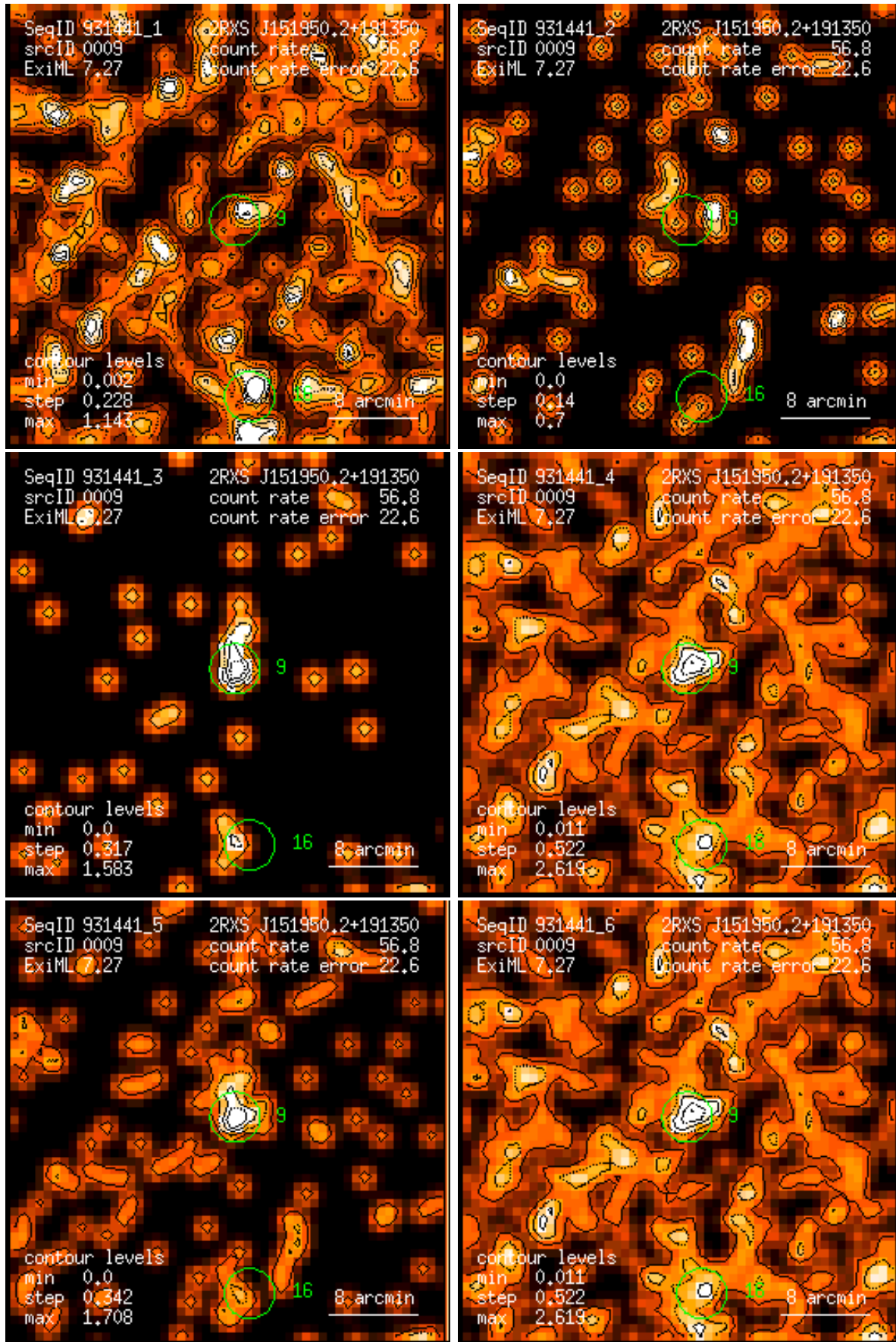
Figure 9: RASS 931441: detection 0009: band rate images, Gaussian filter: (1) PSPC channels 11 – 41, (2) 52 – 90, (3) 91 – 201, (4) 11 – 235, (5) 52 – 201, (6) 11 – 201. Broad band rates in counts/ks. Band rate contour levels in counts/ks/arcmin 2 .
