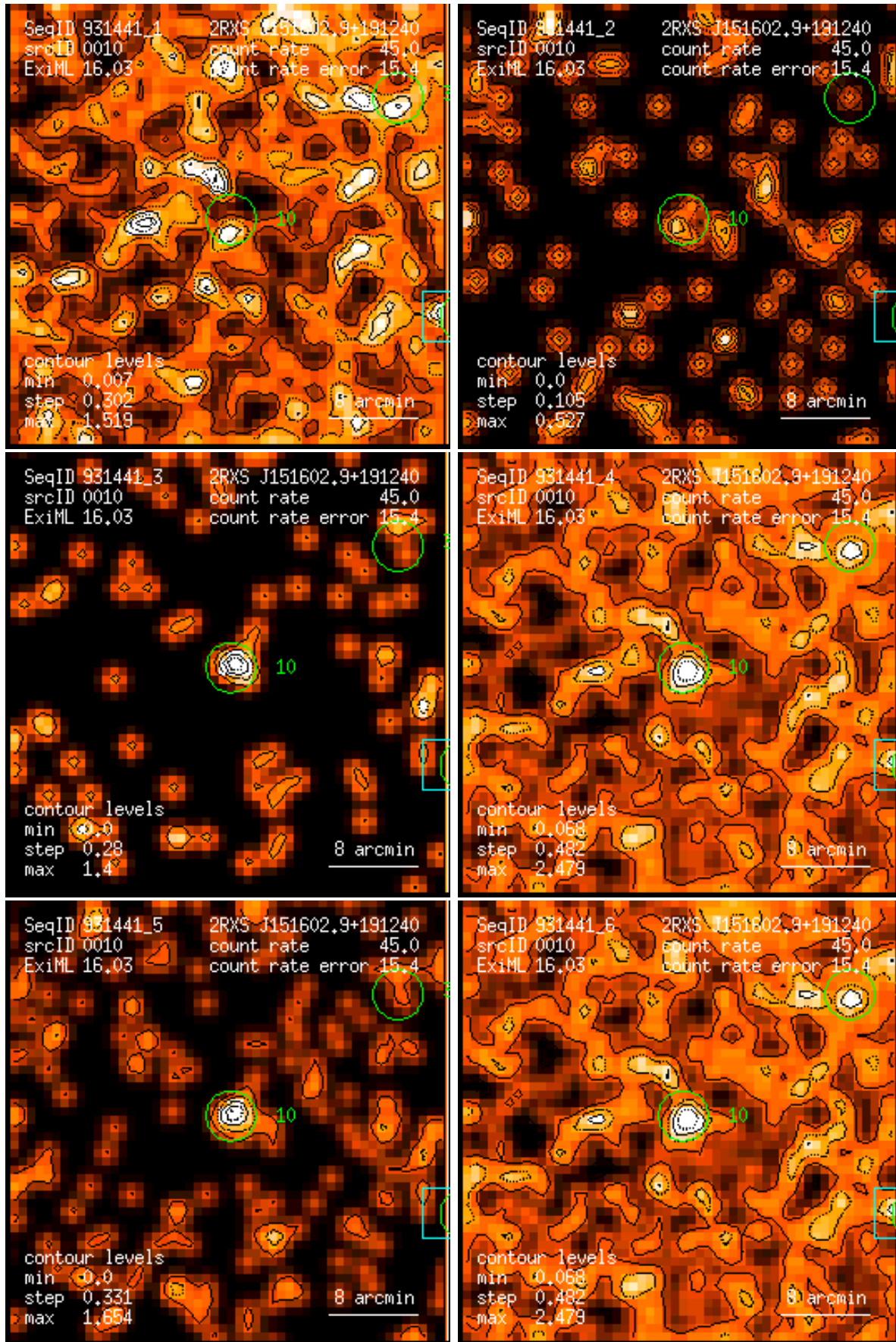
Figure 10: RASS 931441: detection 0010: band rate images, Gaussian filter: (1) PSPC channels 11 – 41, (2) 52 – 90, (3) 91 – 201, (4) 11 – 235, (5) 52 – 201, (6) 11 – 201. Broad band rates in counts/ks. Band rate contour levels in counts/ks/arcmin 2 .
