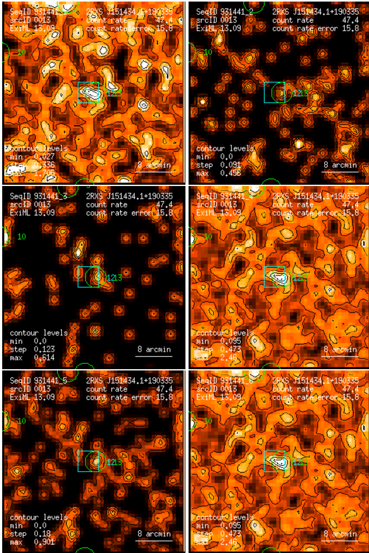
Figure 13: RASS 931441: detection 0013: band rate images, Gaussian filter: (1) PSPC channels 11 – 41, (2) 52 – 90, (3) 91 – 201, (4) 11 – 235, (5) 52 – 201, (6) 11 – 201. Broad band rates in counts/ks. Band rate contour levels in counts/ks/arcmin 2 .
