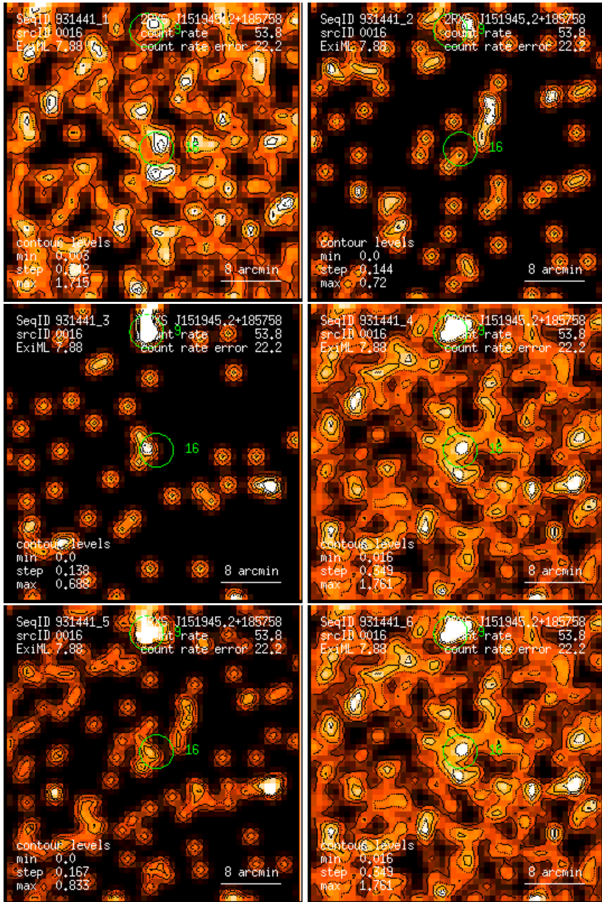
Figure 16: RASS 931441: detection 0016: band rate images, Gaussian filter: (1) PSPC channels 11 – 41, (2) 52 – 90, (3) 91 – 201, (4) 11 – 235, (5) 52 – 201, (6) 11 – 201. Broad band rates in counts/ks. Band rate contour levels in counts/ks/arcmin 2 .
