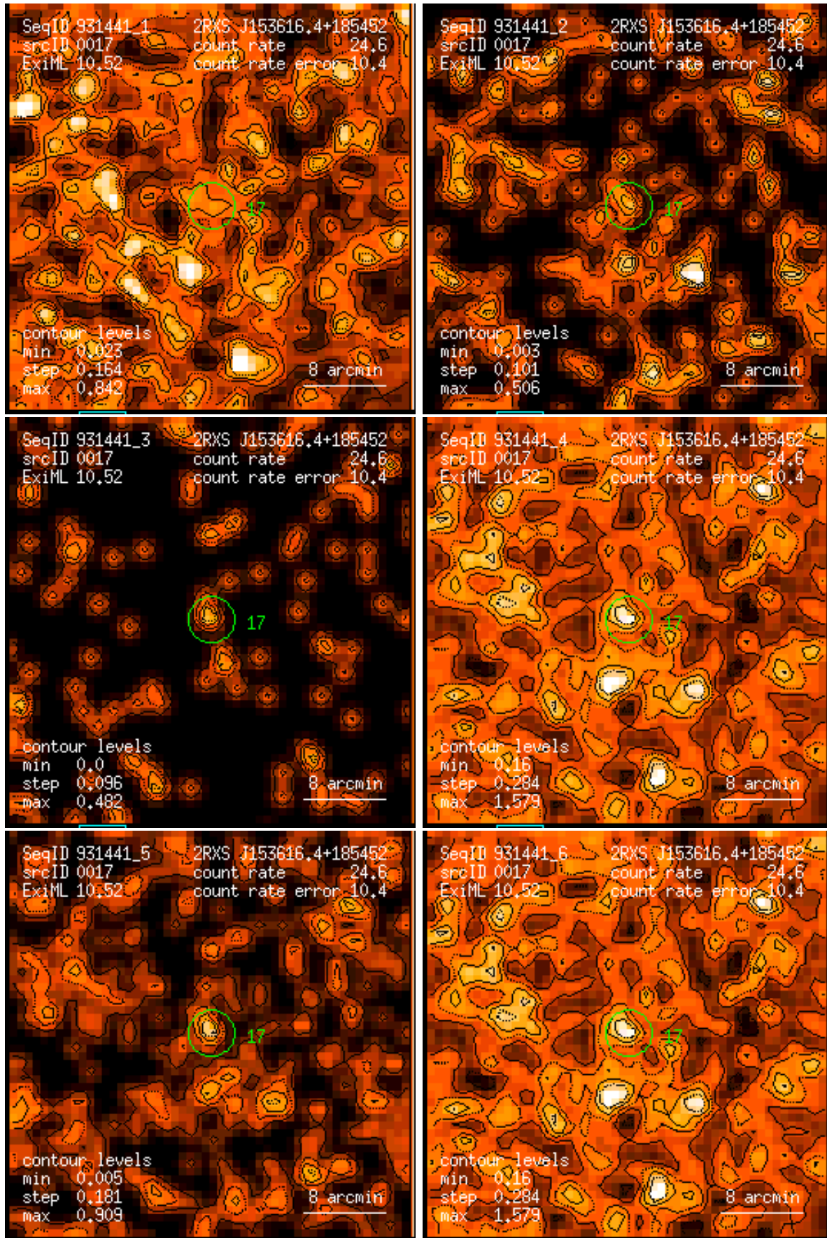
Figure 17: RASS 931441: detection 0017: band rate images, Gaussian filter: (1) PSPC channels 11 – 41, (2) 52 – 90, (3) 91 – 201, (4) 11 – 235, (5) 52 – 201, (6) 11 – 201. Broad band rates in counts/ks. Band rate contour levels in counts/ks/arcmin 2 .
