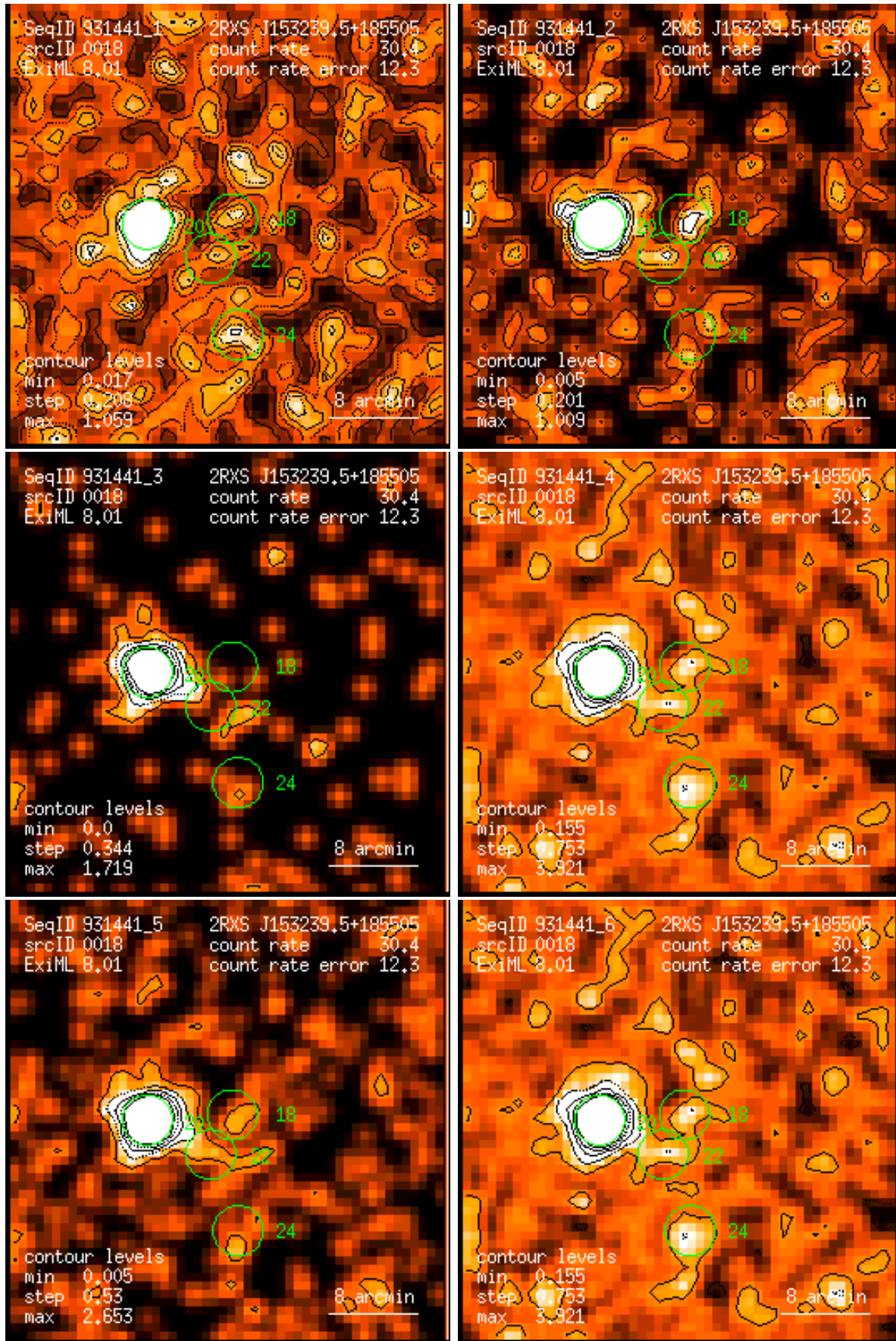
Figure 18: RASS 931441: detection 0018: band rate images, Gaussian filter: (1) PSPC channels 11 – 41, (2) 52 – 90, (3) 91 – 201, (4) 11 – 235, (5) 52 – 201, (6) 11 – 201. Broad band rates in counts/ks. Band rate contour levels in counts/ks/arcmin 2 .
