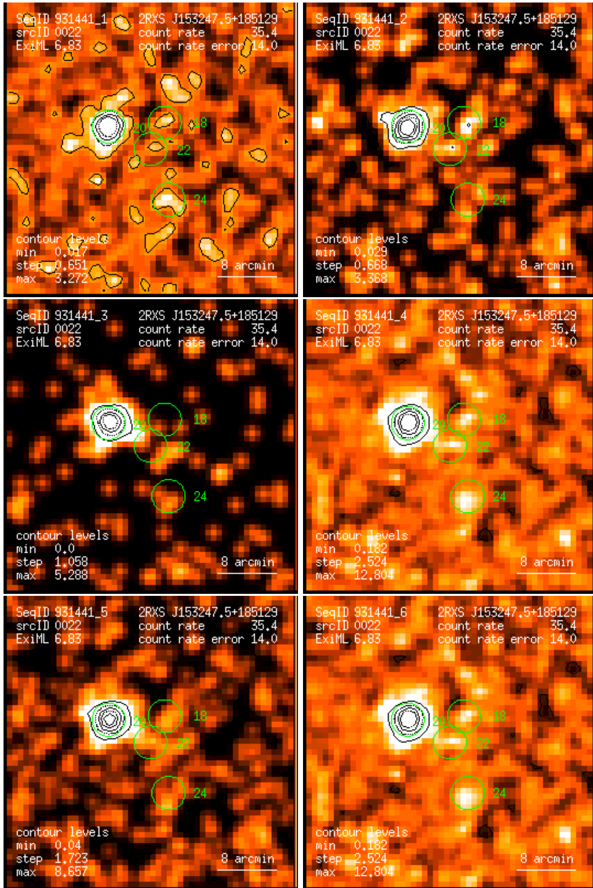
Figure 22: RASS 931441: detection 0022: band rate images, Gaussian filter: (1) PSPC channels 11 – 41, (2) 52 – 90, (3) 91 – 201, (4) 11 – 235, (5) 52 – 201, (6) 11 – 201. Broad band rates in counts/ks. Band rate contour levels in counts/ks/arcmin 2 .
