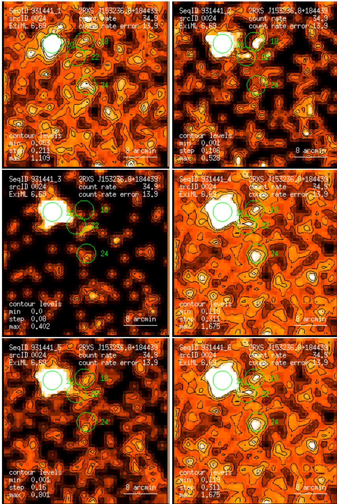
Figure 24: RASS 931441: detection 0024: band rate images, Gaussian filter: (1) PSPC channels 11 – 41, (2) 52 – 90, (3) 91 – 201, (4) 11 – 235, (5) 52 – 201, (6) 11 – 201. Broad band rates in counts/ks. Band rate contour levels in counts/ks/arcmin 2 .
