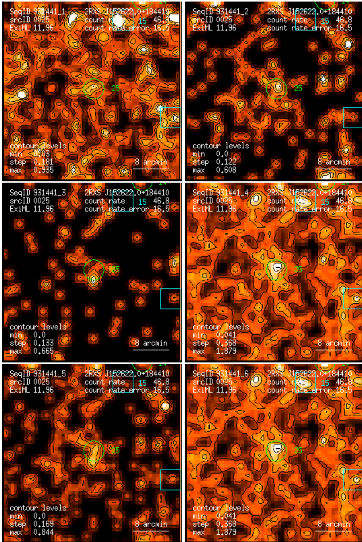
Figure 25: RASS 931441: detection 0025: band rate images, Gaussian filter: (1) PSPC channels 11 – 41, (2) 52 – 90, (3) 91 – 201, (4) 11 – 235, (5) 52 – 201, (6) 11 – 201. Broad band rates in counts/ks. Band rate contour levels in counts/ks/arcmin 2 .
