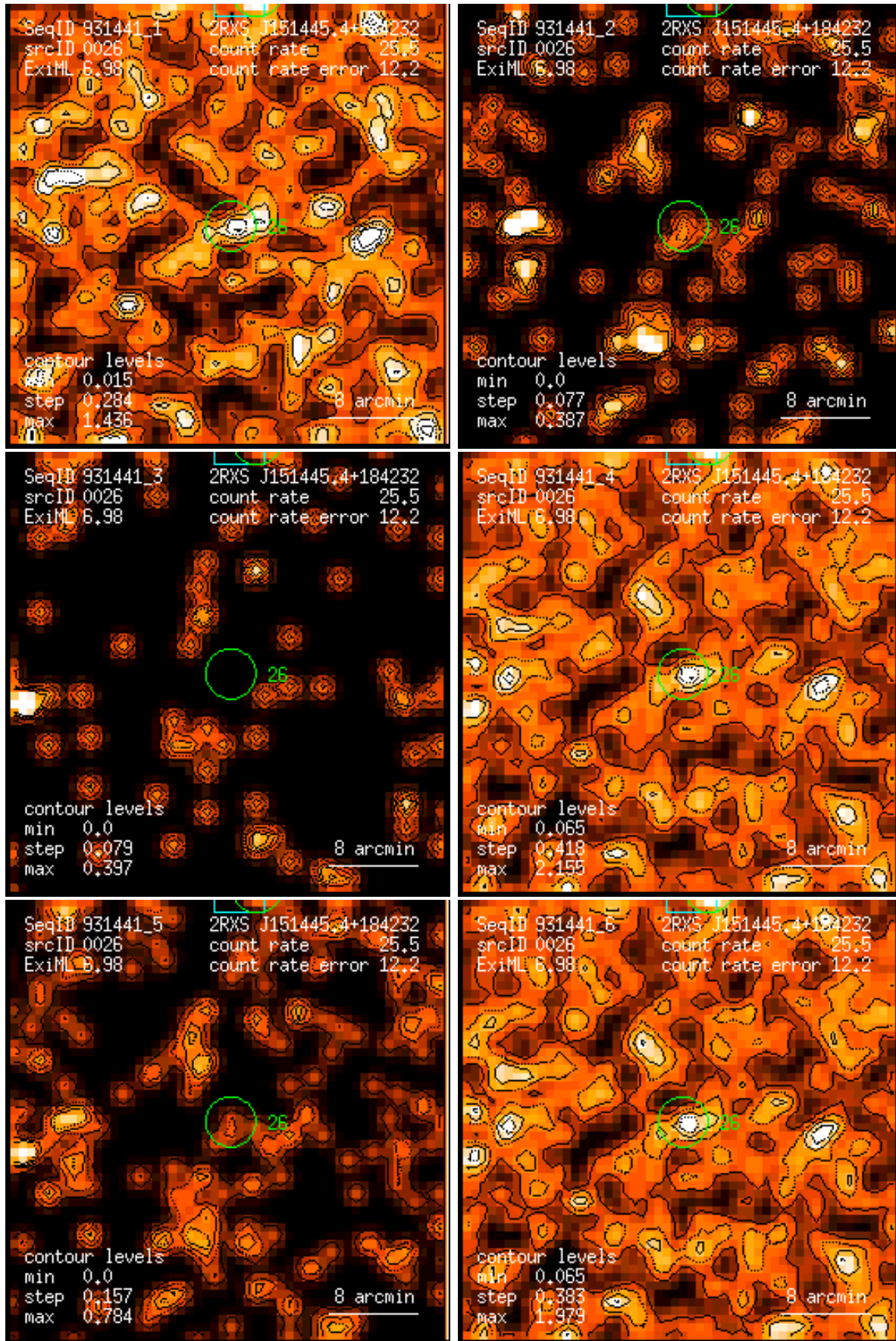
Figure 26: RASS 931441: detection 0026: band rate images, Gaussian filter: (1) PSPC channels 11 – 41, (2) 52 – 90, (3) 91 – 201, (4) 11 – 235, (5) 52 – 201, (6) 11 – 201. Broad band rates in counts/ks. Band rate contour levels in counts/ks/arcmin 2 .
