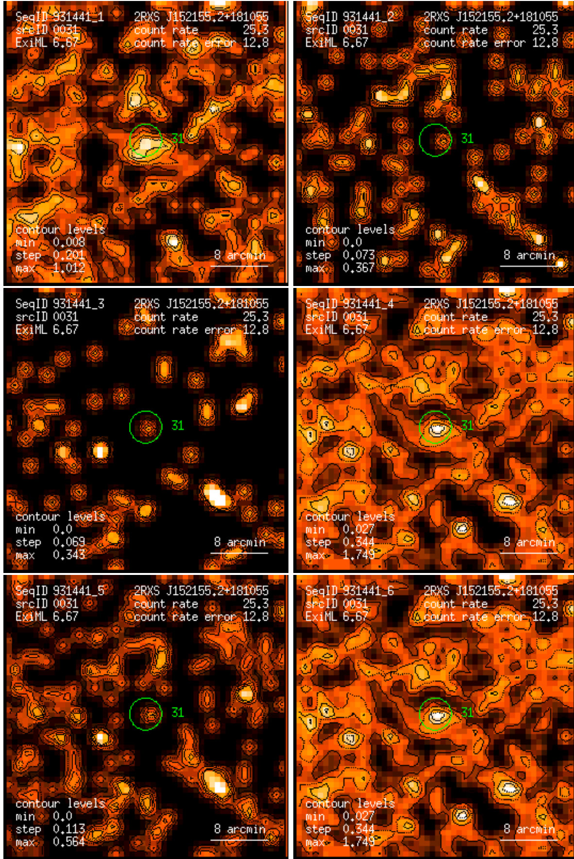
Figure 31: RASS 931441: detection 0031: band rate images, Gaussian filter: (1) PSPC channels 11 – 41, (2) 52 – 90, (3) 91 – 201, (4) 11 – 235, (5) 52 – 201, (6) 11 – 201. Broad band rates in counts/ks. Band rate contour levels in counts/ks/arcmin 2 .
