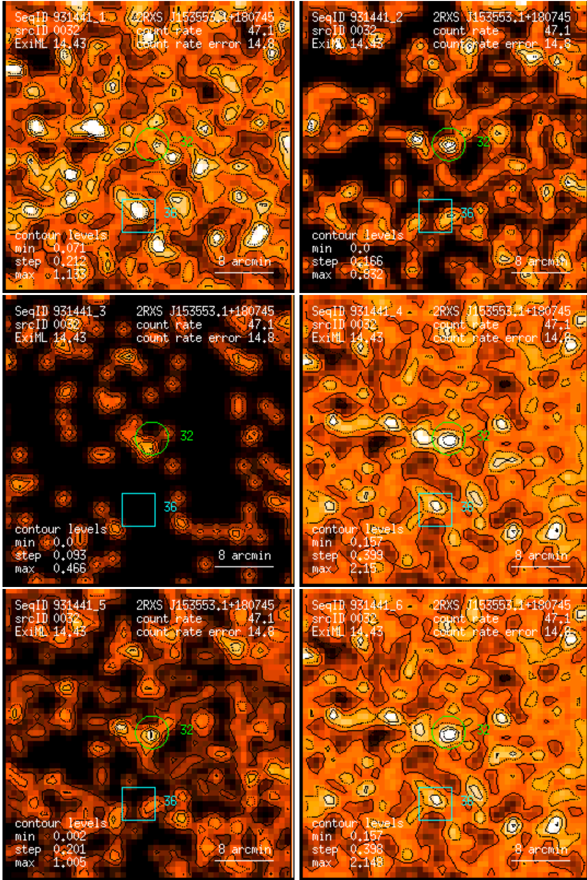
Figure 32: RASS 931441: detection 0032: band rate images, Gaussian filter: (1) PSPC channels 11 – 41, (2) 52 – 90, (3) 91 – 201, (4) 11 – 235, (5) 52 – 201, (6) 11 – 201. Broad band rates in counts/ks. Band rate contour levels in counts/ks/arcmin 2 .
