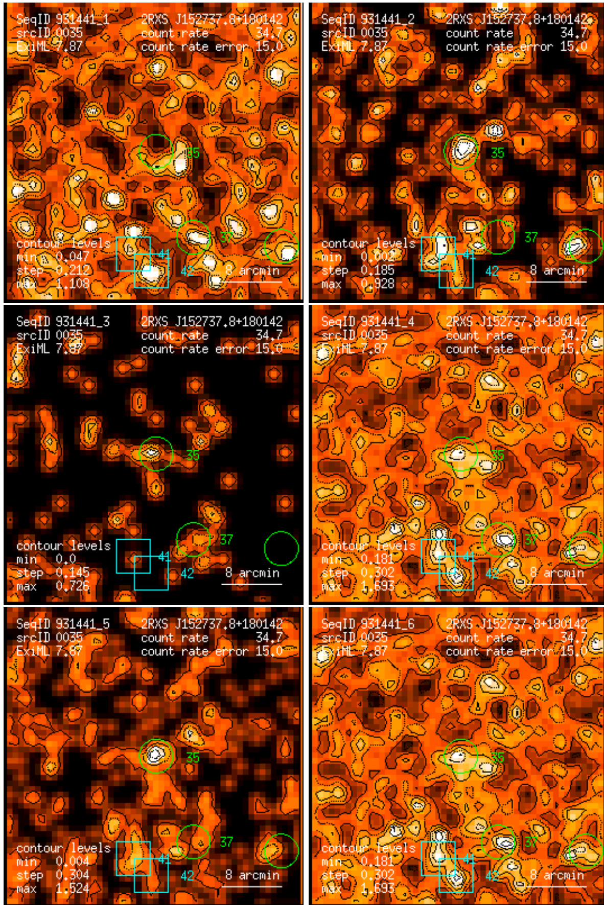
Figure 35: RASS 931441: detection 0035: band rate images, Gaussian filter: (1) PSPC channels 11 – 41, (2) 52 – 90, (3) 91 – 201, (4) 11 – 235, (5) 52 – 201, (6) 11 – 201. Broad band rates in counts/ks. Band rate contour levels in counts/ks/arcmin 2 .
