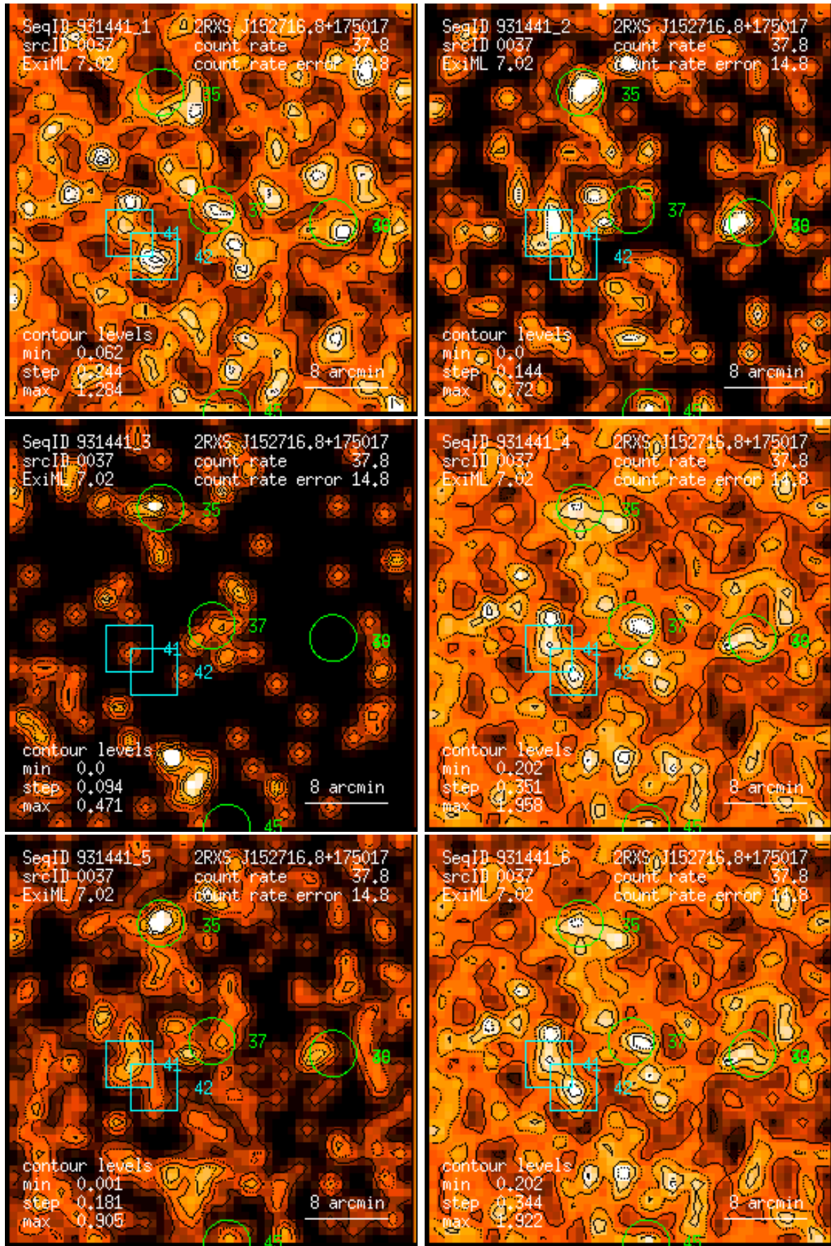
Figure 37: RASS 931441: detection 0037: band rate images, Gaussian filter: (1) PSPC channels 11 – 41, (2) 52 – 90, (3) 91 – 201, (4) 11 – 235, (5) 52 – 201, (6) 11 – 201. Broad band rates in counts/ks. Band rate contour levels in counts/ks/arcmin 2 .
