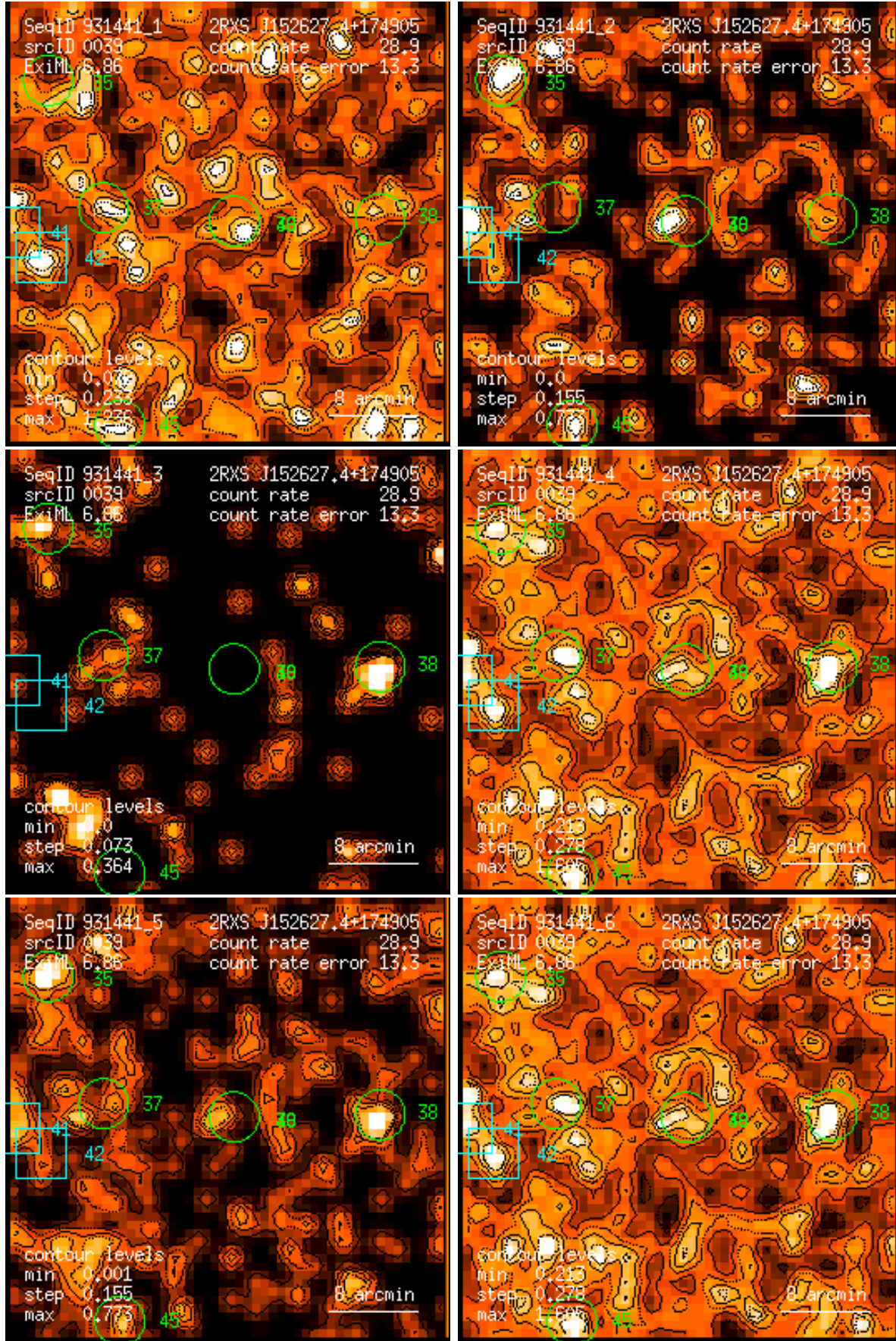
Figure 39: RASS 931441: detection 0039: band rate images, Gaussian filter: (1) PSPC channels 11 – 41, (2) 52 – 90, (3) 91 – 201, (4) 11 – 235, (5) 52 – 201, (6) 11 – 201. Broad band rates in counts/ks. Band rate contour levels in counts/ks/arcmin 2 .
