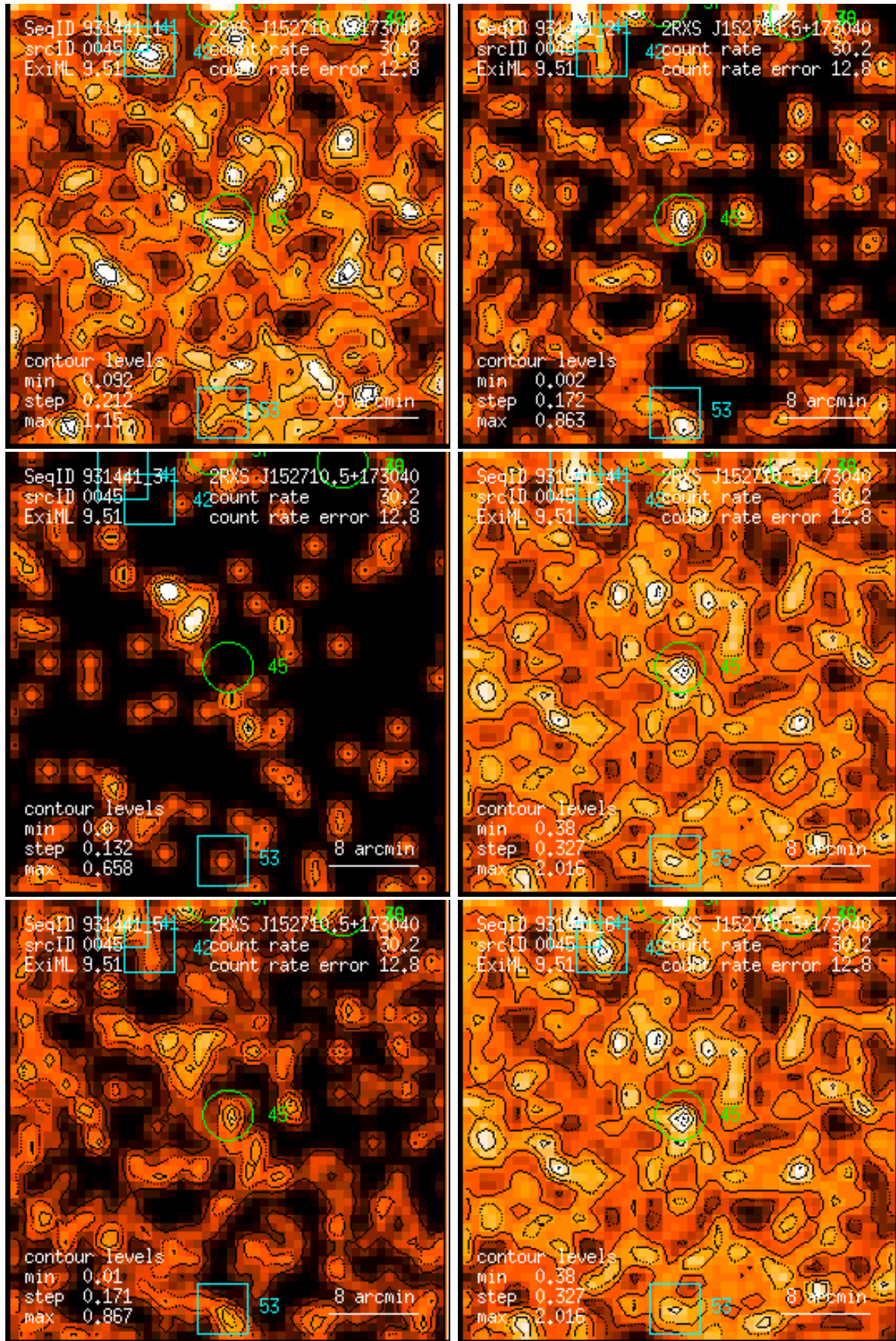
Figure 45: RASS 931441: detection 0045: band rate images, Gaussian filter: (1) PSPC channels 11 – 41, (2) 52 – 90, (3) 91 – 201, (4) 11 – 235, (5) 52 – 201, (6) 11 – 201. Broad band rates in counts/ks. Band rate contour levels in counts/ks/arcmin 2 .
