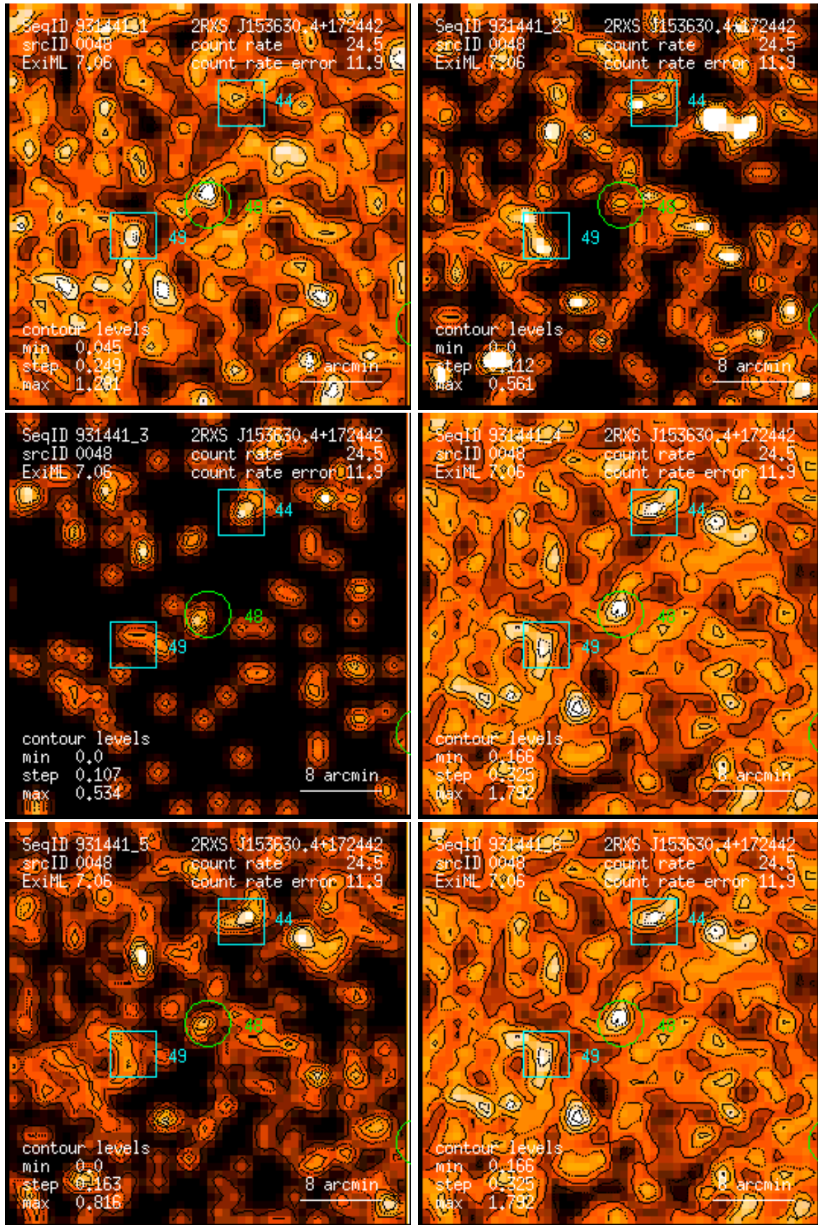
Figure 48: RASS 931441: detection 0048: band rate images, Gaussian filter: (1) PSPC channels 11 – 41, (2) 52 – 90, (3) 91 – 201, (4) 11 – 235, (5) 52 – 201, (6) 11 – 201. Broad band rates in counts/ks. Band rate contour levels in counts/ks/arcmin 2 .
