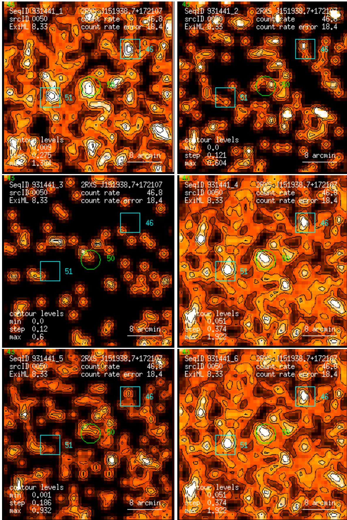
Figure 50: RASS 931441: detection 0050: band rate images, Gaussian filter: (1) PSPC channels 11 – 41, (2) 52 – 90, (3) 91 – 201, (4) 11 – 235, (5) 52 – 201, (6) 11 – 201. Broad band rates in counts/ks. Band rate contour levels in counts/ks/arcmin 2 .
