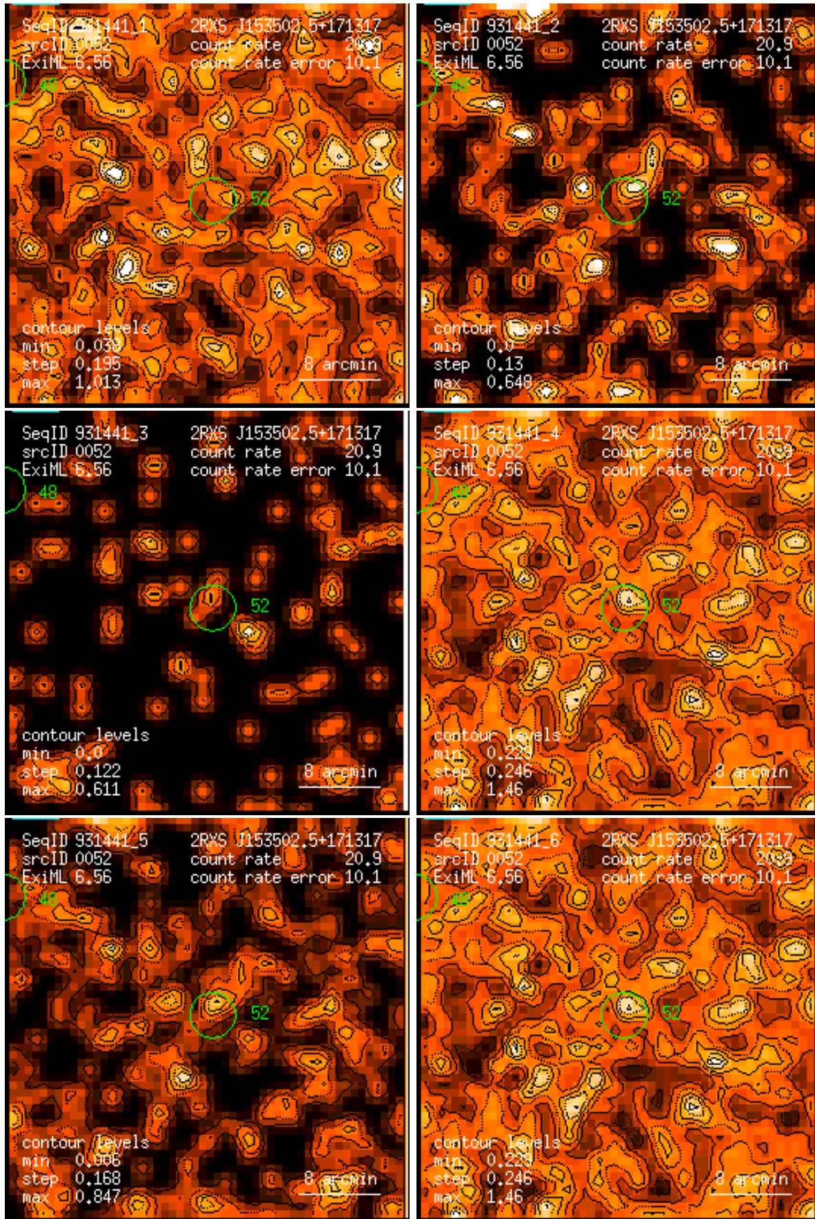
Figure 52: RASS 931441: detection 0052: band rate images, Gaussian filter: (1) PSPC channels 11 – 41, (2) 52 – 90, (3) 91 – 201, (4) 11 – 235, (5) 52 – 201, (6) 11 – 201. Broad band rates in counts/ks. Band rate contour levels in counts/ks/arcmin 2 .
