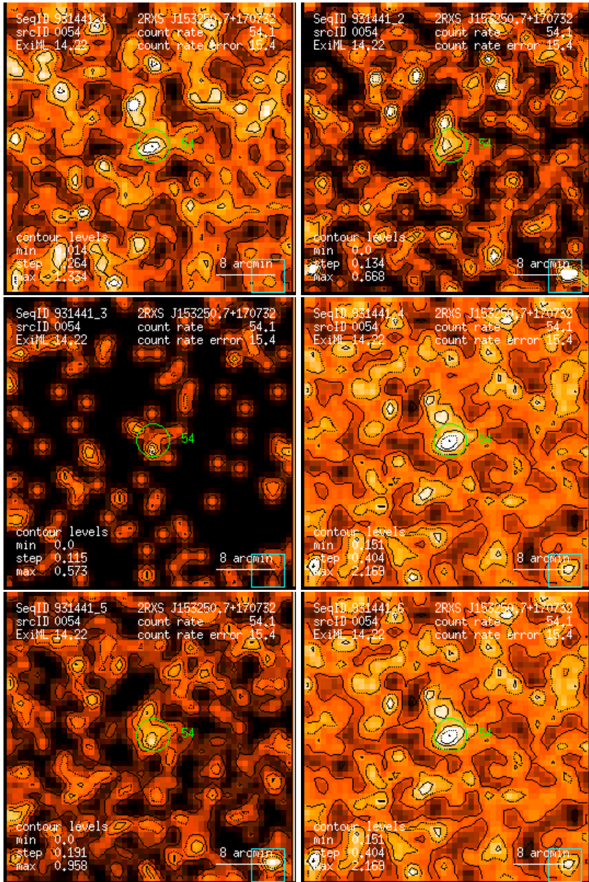
Figure 54: RASS 931441: detection 0054: band rate images, Gaussian filter: (1) PSPC channels 11 – 41, (2) 52 – 90, (3) 91 – 201, (4) 11 – 235, (5) 52 – 201, (6) 11 – 201. Broad band rates in counts/ks. Band rate contour levels in counts/ks/arcmin 2 .
