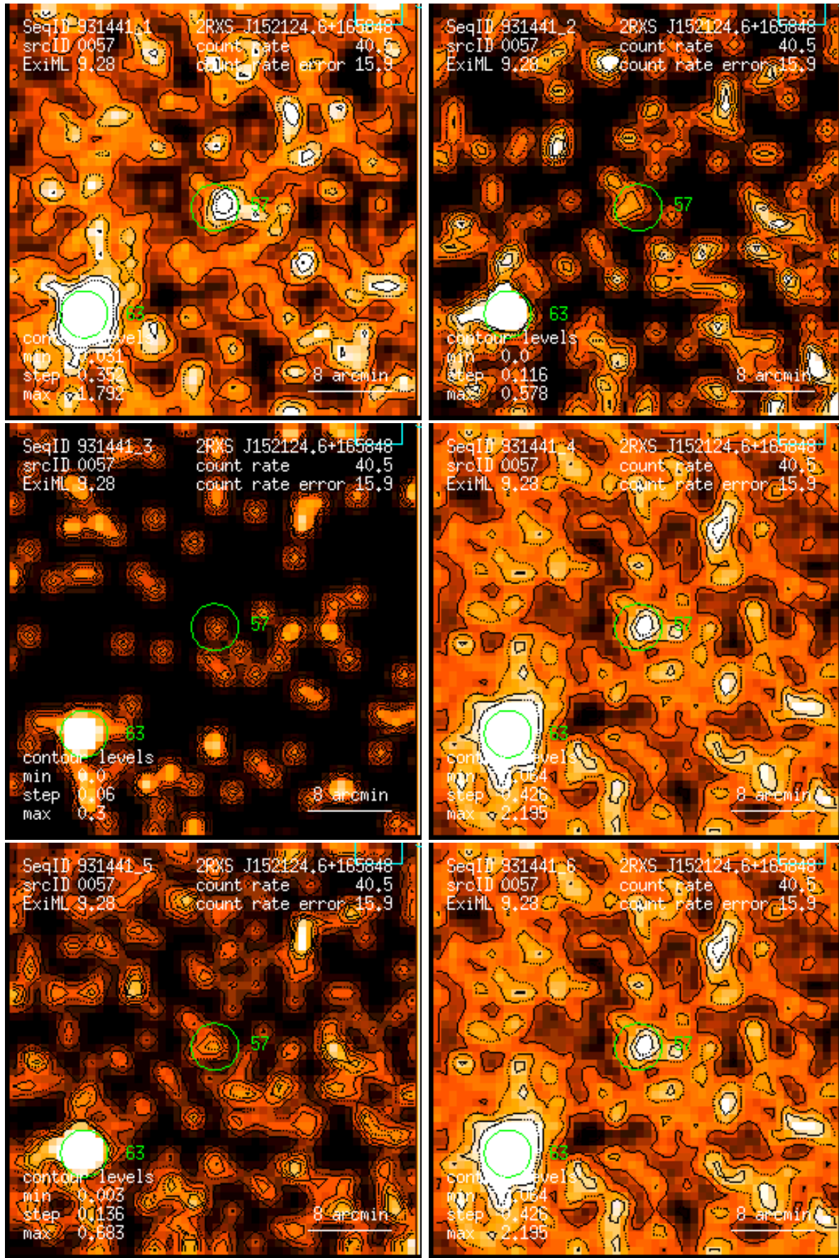
Figure 57: RASS 931441: detection 0057: band rate images, Gaussian filter: (1) PSPC channels 11 – 41, (2) 52 – 90, (3) 91 – 201, (4) 11 – 235, (5) 52 – 201, (6) 11 – 201. Broad band rates in counts/ks. Band rate contour levels in counts/ks/arcmin 2 .
