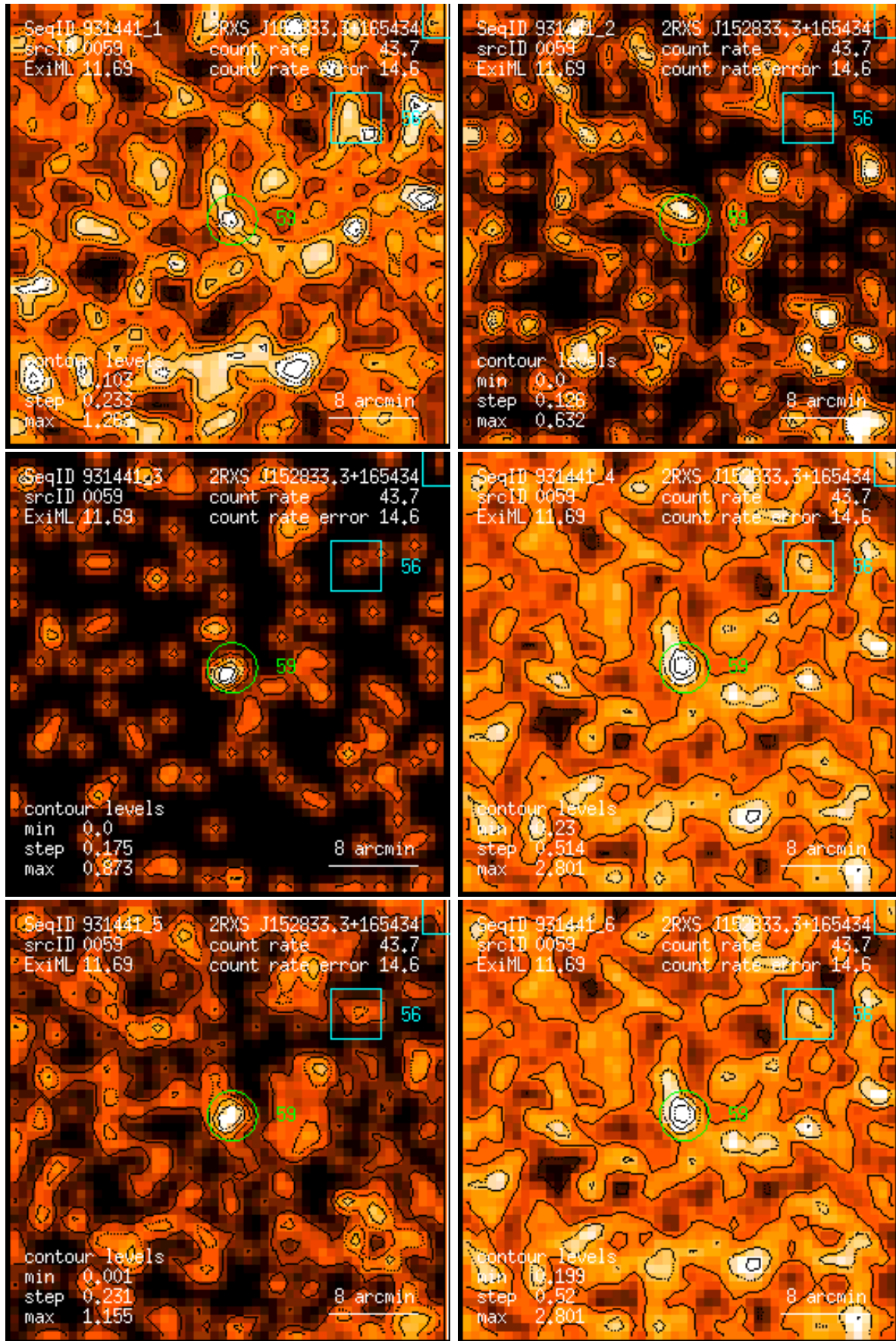
Figure 59: RASS 931441: detection 0059: band rate images, Gaussian filter: (1) PSPC channels 11 – 41, (2) 52 – 90, (3) 91 – 201, (4) 11 – 235, (5) 52 – 201, (6) 11 – 201. Broad band rates in counts/ks. Band rate contour levels in counts/ks/arcmin 2 .
