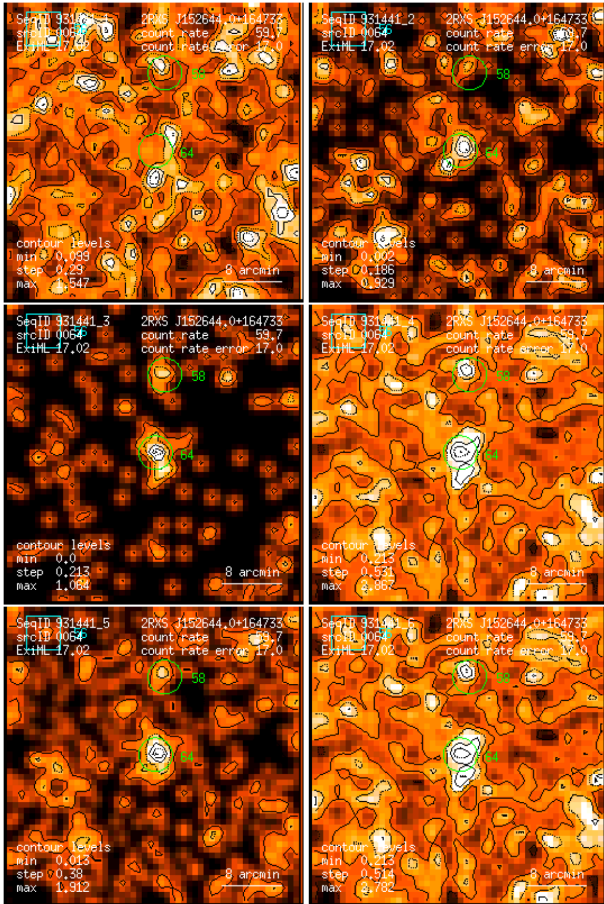
Figure 64: RASS 931441: detection 0064: band rate images, Gaussian filter: (1) PSPC channels 11 – 41, (2) 52 – 90, (3) 91 – 201, (4) 11 – 235, (5) 52 – 201, (6) 11 – 201. Broad band rates in counts/ks. Band rate contour levels in counts/ks/arcmin 2 .
