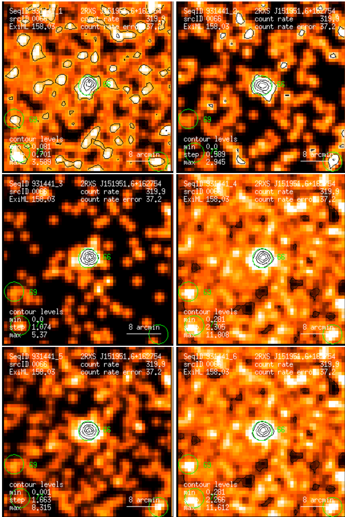
Figure 66: RASS 931441: detection 0066: band rate images, Gaussian filter: (1) PSPC channels 11 – 41, (2) 52 – 90, (3) 91 – 201, (4) 11 – 235, (5) 52 – 201, (6) 11 – 201. Broad band rates in counts/ks. Band rate contour levels in counts/ks/arcmin 2 .
