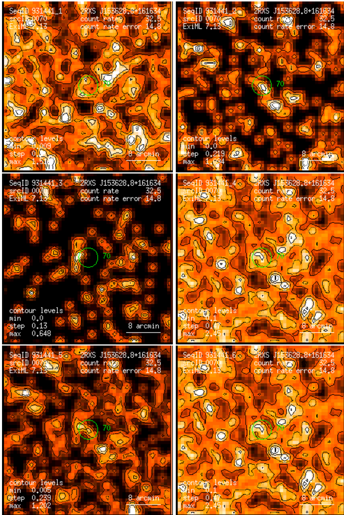
Figure 70: RASS 931441: detection 0070: band rate images, Gaussian filter: (1) PSPC channels 11 – 41, (2) 52 – 90, (3) 91 – 201, (4) 11 – 235, (5) 52 – 201, (6) 11 – 201. Broad band rates in counts/ks. Band rate contour levels in counts/ks/arcmin 2 .
