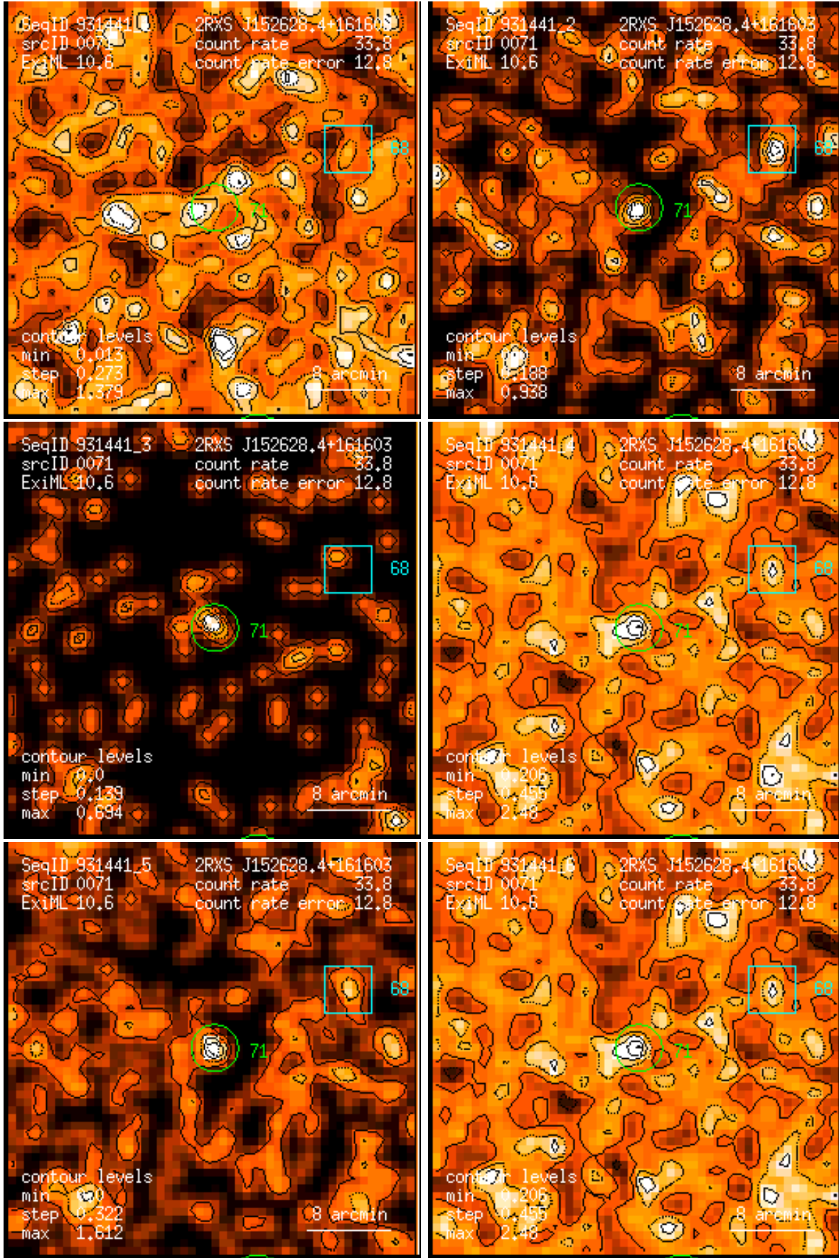
Figure 71: RASS 931441: detection 0071: band rate images, Gaussian filter: (1) PSPC channels 11 – 41, (2) 52 – 90, (3) 91 – 201, (4) 11 – 235, (5) 52 – 201, (6) 11 – 201. Broad band rates in counts/ks. Band rate contour levels in counts/ks/arcmin 2 .
